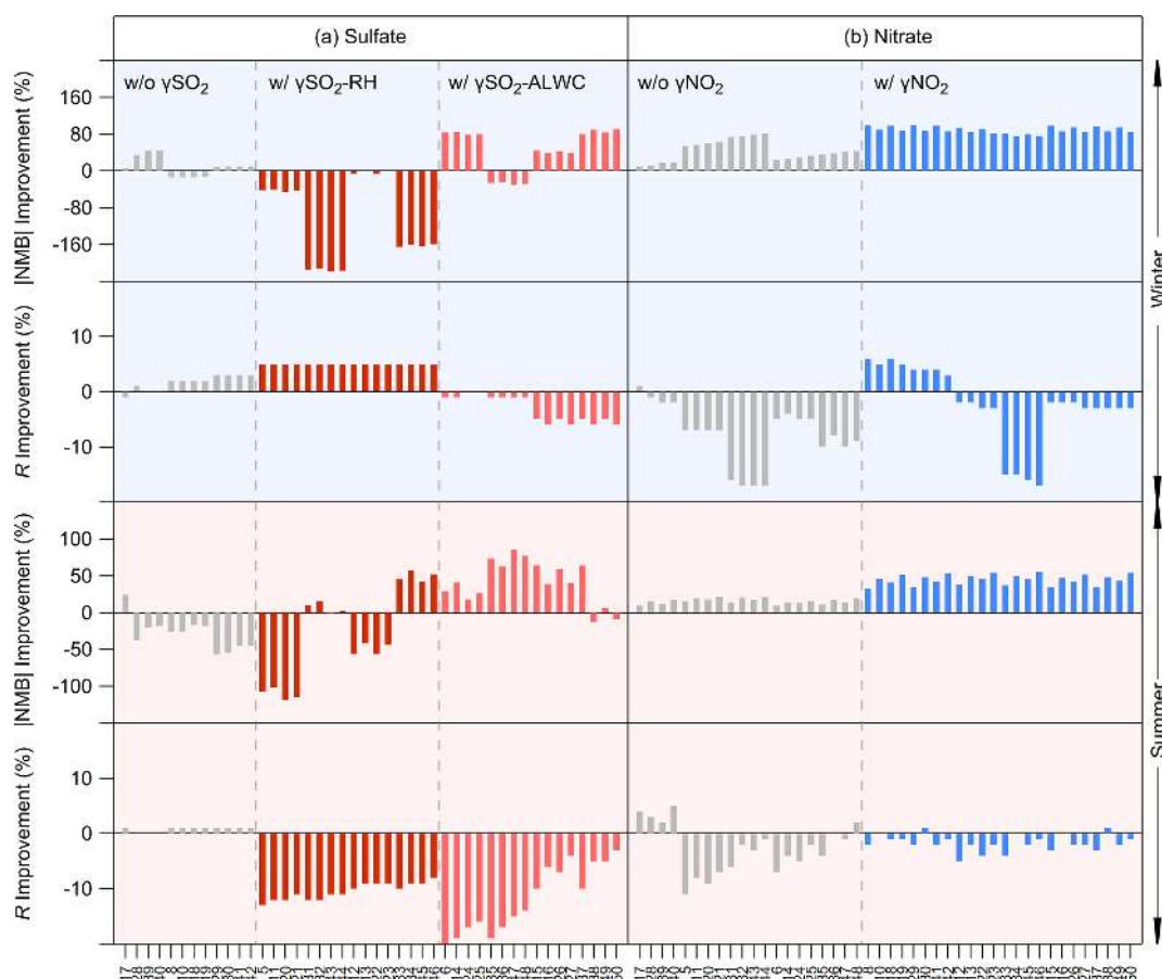
Figure 7. The improvements of the R and the |NMB| values for (a) sulfate and (b) nitrate in Cases 10–50 relative to Case 0 (standard) during the selected wintertime and summertime periods. For comparison, Cases 5 (with \gamma_{SO_2-RH} ), 6 (with \gamma_{SO_2-ALWC} ), and 8 (reduced \gamma_{NO_2} ) are also plotted. Positive values in |NMB| or R improvement mean improved simulations.
