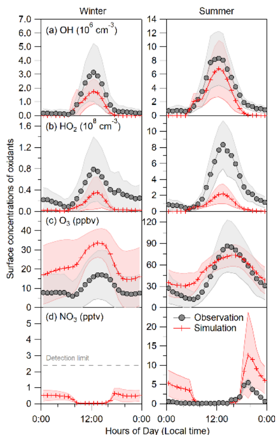
Figure 5. Diurnal profiles of the hourly mean simulated and observed concentrations of (a) OH• and (b) HO 2 • at the Wangdu site from June to July 2014 and at the Huairou site from January to March 2016, (c) O 3 at the PKUERS site from July 2011 to May 2013, and (d) NO 3 • at the PKUERS site in January and September 2016 in Beijing. The shaded areas indicate mean value ± 1 standard deviation.
