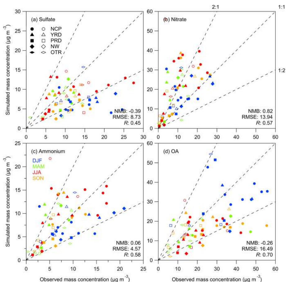
Figure 1. Scatterplots of the simulated and observed campaign-average mass concentrations of (a) sulfate, (b) nitrate, (c) ammonium, and (d) OA in China. The solid and open symbols represent the urban and non-urban sites, respectively. Colors and shapes of the symbols represent seasons and regions, respectively. The observations were conducted during 2006 to 2016 for submicron particles, and the data were divided by a submicron-to-fine ratio of 0.8. The model simulations were run for the year 2012.
