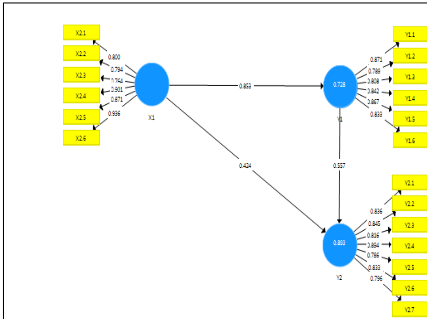
Figure 2. PLS Algorithm
