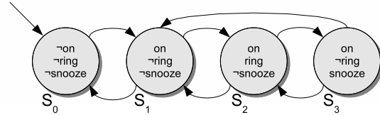
Fig. 1. The Kripke structure of an alarm clock
