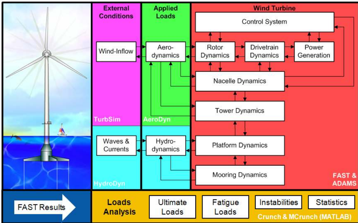
Figure 2. FAST modules
