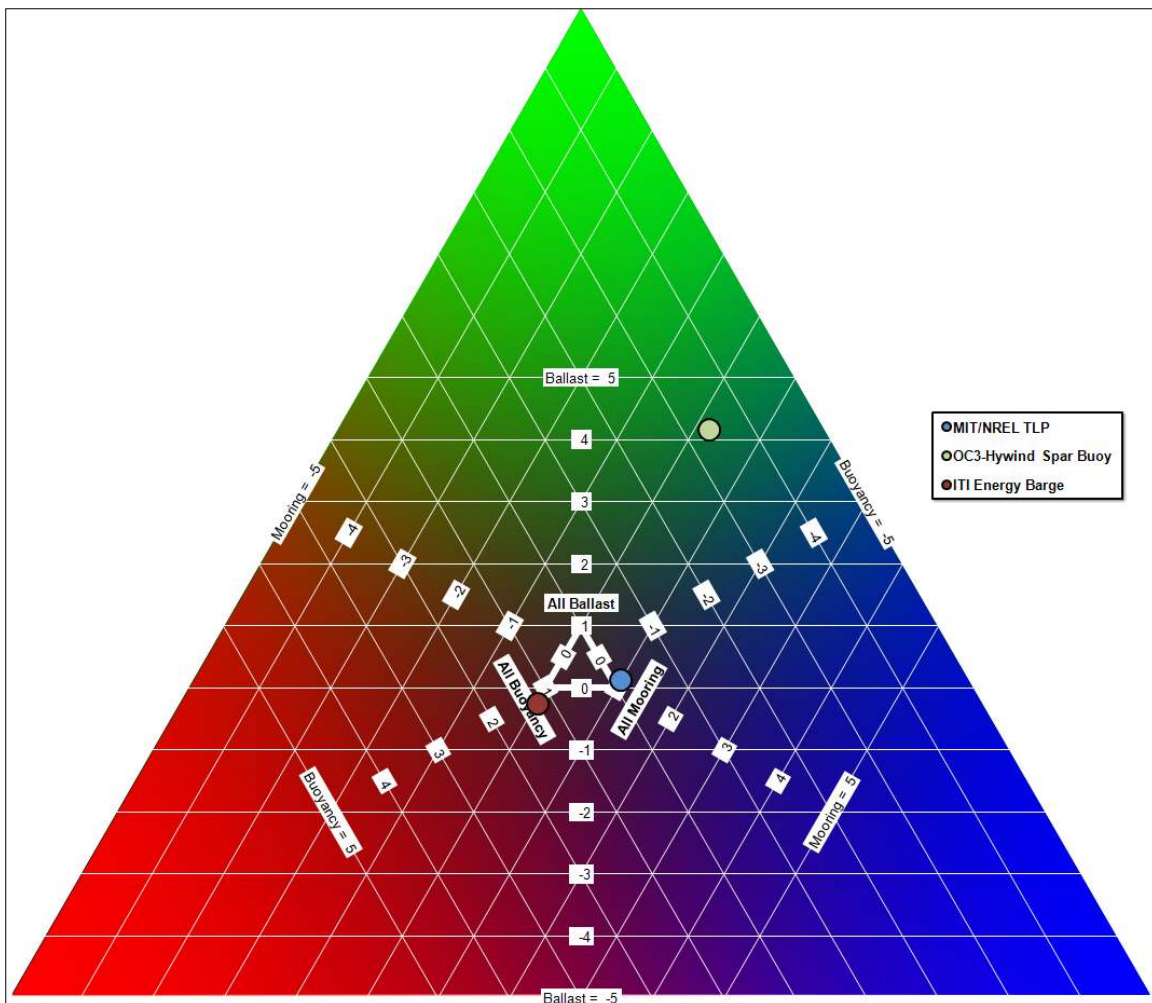
Figure 48. Floating wind turbines stability triangle (ternary plot)
