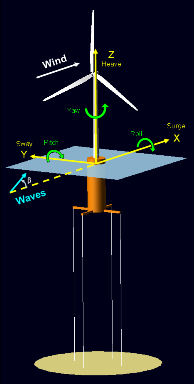
Figure 6. Coordinate system
