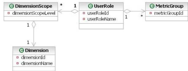
Figure 7: UserRole to Metric and Dimension model.
