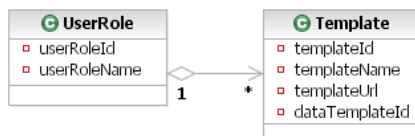
Figure 8: UserRole to report Template model.
