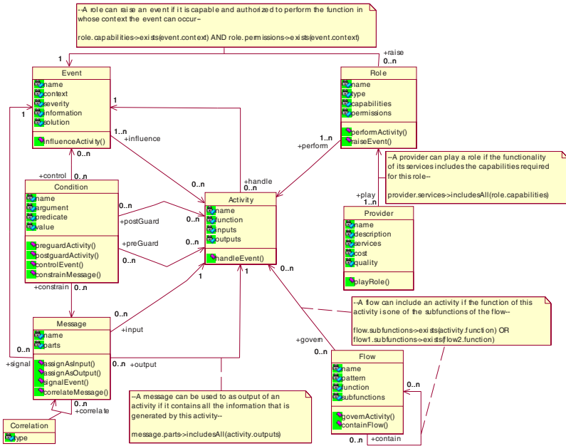
Fig. 2. Service composition model
