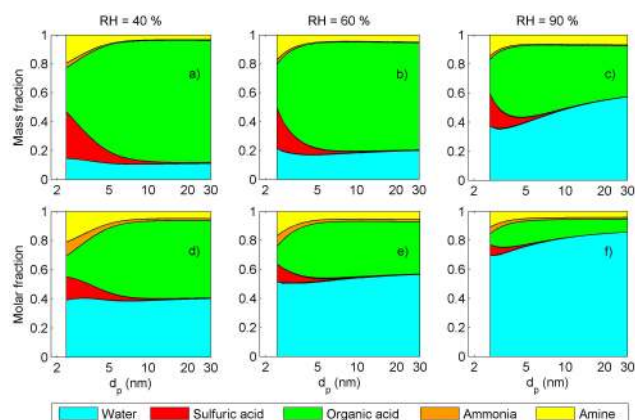
Fig. 7. Mass (a, b, c) and molar (d, e, f) fractions as a function of particle size in simulations where RH was 40% (a, d), 60% (b, e) and 90% (c, f). Concentrations of sulfuric acid ( 10^6 \text{ cm}^{-3} ), ammonia ( 10^9 \text{ cm}^{-3} ) and amine ( 10^9 \text{ cm}^{-3} ), RH (40%) and temperature (283.15 K) were set to base case values. Concentration of organic acid was 3 \times 10^8 \text{ cm}^{-3} and p_{\text{sat, Org. acid}} was 10^{-6} \text{ Pa} .
