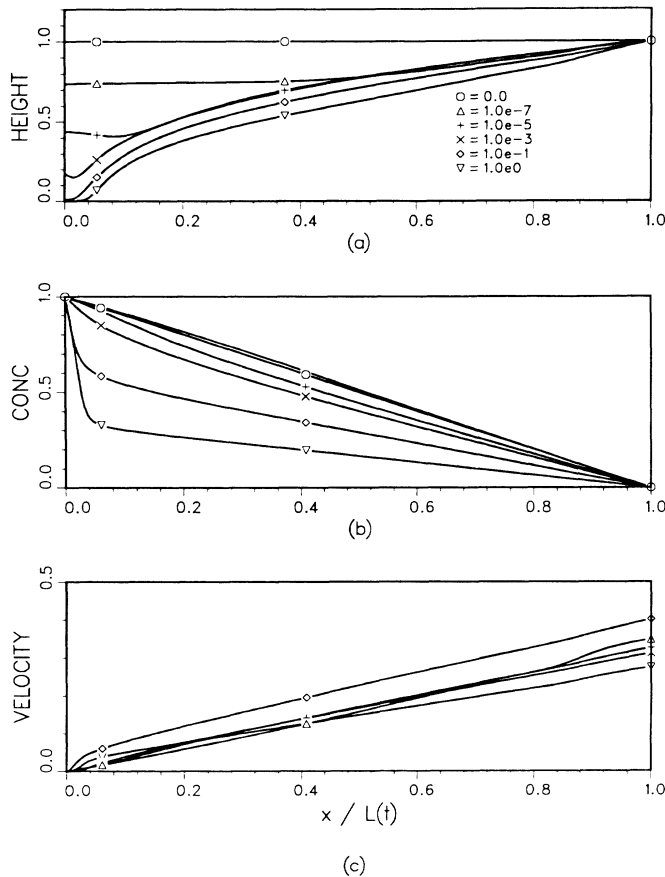
FIG. 2. The profiles in region 3 for the (a) height h/2b , (b) concentration \Gamma/\Gamma_{\text{drop}} , and (c) relative surface velocity (U - U_{\text{rel}})/[L(\tau)/t_L] , as functions of \tau = t/t_L , where t_L = 72(\alpha\Gamma_{\text{drop}}/\sigma_{\text{drop}})(\eta b/\sigma_{\text{drop}})[S/\theta(0)]^3 .
