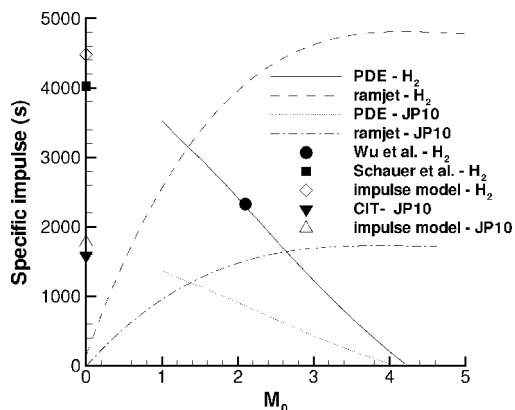
Fig. 11 Specific impulse of single-tube airbreathing PDE compared to ideal ramjet operating with stoichiometric hydrogen–air and JP10–air at altitude of 10 km.
