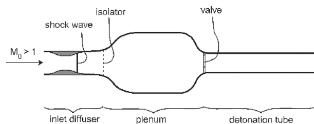
Fig. 1 Schematic of single-tube PDE.
