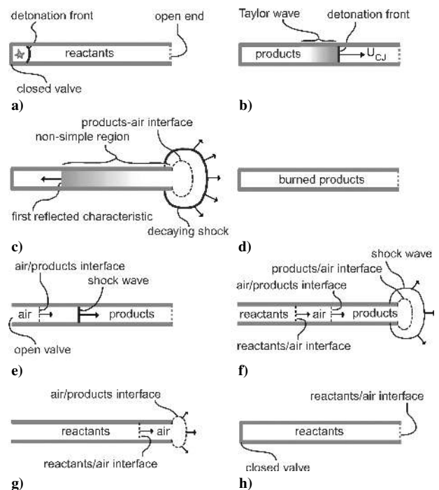
Fig. 3 PDE cycle schematic for single detonation tube.
