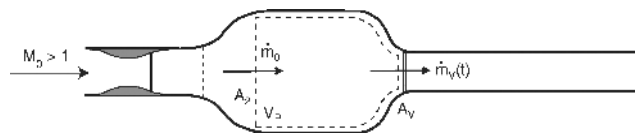
Fig. 4 Control volume V_P used for analysis of flow in plenum.
