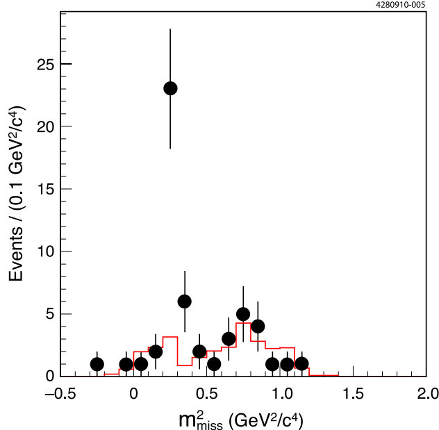
FIG. 7: Missing-mass squared distribution for CP -tagged D^0 \rightarrow K_S^0 K^+ K^- candidates where the CP -eigenstate contains a K_L^0 meson. The points are data and the solid histogram is the background estimated from simulation.
