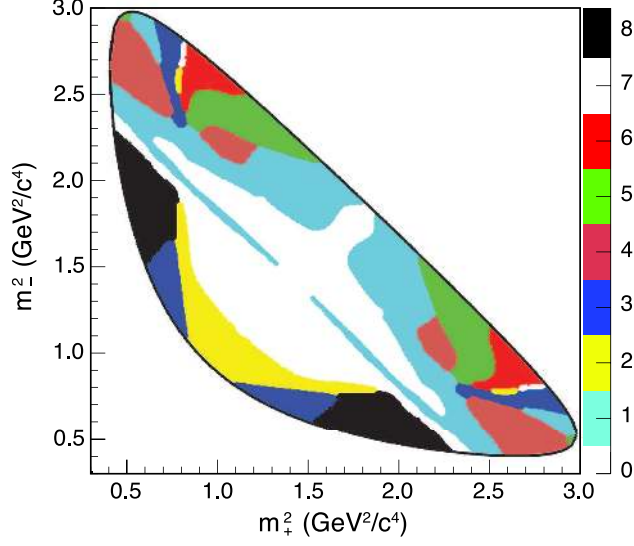
FIG. 4: Modified-optimal binning of the D^0 \rightarrow K_S^0 \pi^+ \pi^- Dalitz plot based on the BABAR 2008 model. The color scale represents the absolute value of the bin number, |i| .
