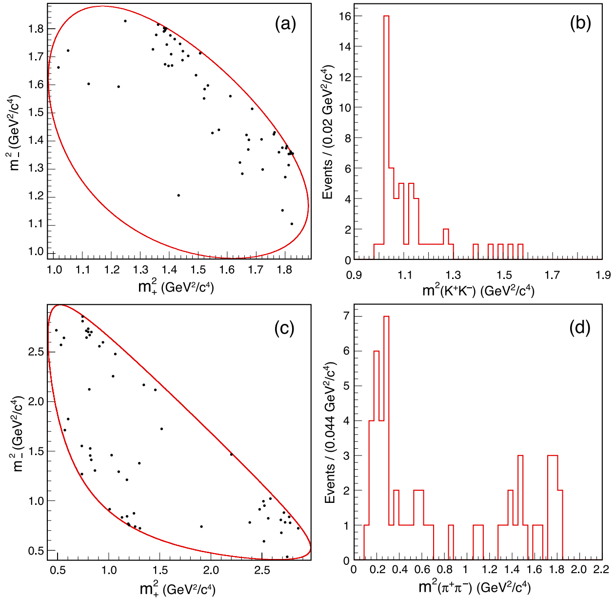
FIG. 11: (a) Dalitz plot and (b) m_{K^+K^-}^2 distributions of D^0 \rightarrow K_S^0 K^+ K^- candidates tagged by \bar{D}^0 \rightarrow K_S^0 \pi^+ \pi^- decays. (c) Dalitz plot and (d) m_{\pi^+\pi^-}^2 distributions of the D^0 \rightarrow K_S^0 \pi^+ \pi^- candidates in the same events.
