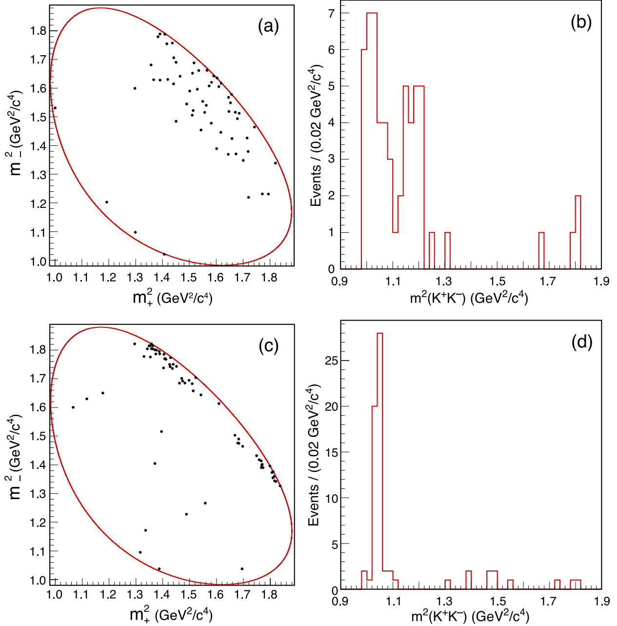
FIG. 10: (a) Dalitz plot and (b) m_{K^+K^-}^2 distributions of D^0 \rightarrow K_L^0 K^+ K^- candidates tagged by a CP -even eigenstate. (c) Dalitz plot and (d) m_{K^+K^-}^2 distributions of D^0 \rightarrow K_L^0 K^+ K^- candidates tagged by a CP -odd eigenstate.
