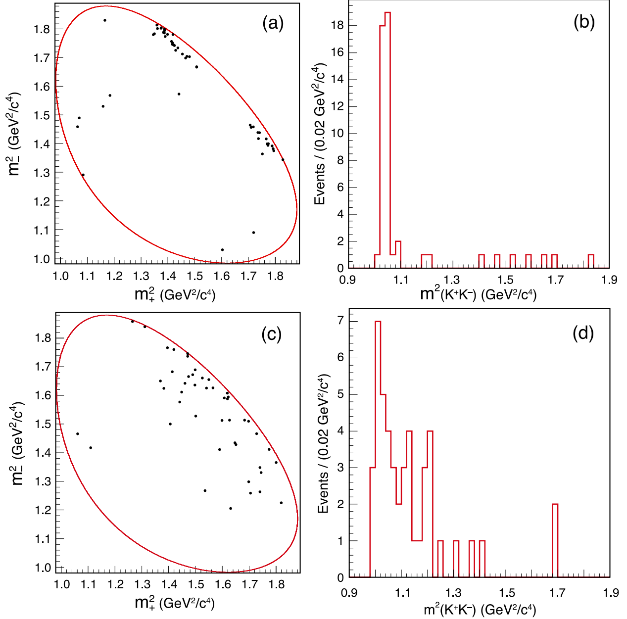
FIG. 9: (a) Dalitz plot and (b) m_{K^+K^-}^2 distributions of D^0 \rightarrow K_S^0 K^+ K^- candidates tagged by a CP -even eigenstate. (c) Dalitz plot and (d) m_{K^+K^-}^2 distributions of D^0 \rightarrow K_S^0 K^+ K^- candidates tagged by a CP -odd eigenstate.
