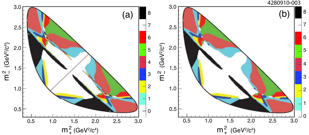
FIG. 3: (a) Optimal binning of the D^0 \rightarrow K_S^0 \pi^+ \pi^- Dalitz plot that was found to exploit best the B -statistics according to the BABAR 2008 model. (b) The same binning after the smoothing procedure described in the text has been applied. The color scale represents the value |z| .
