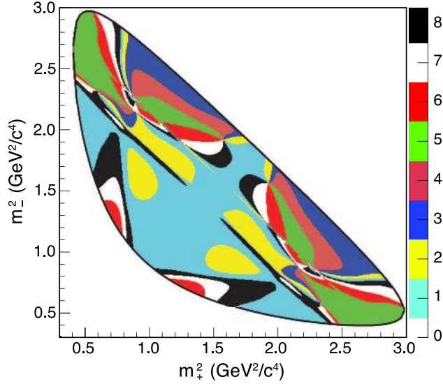
FIG. 5: Equal \Delta\delta_D binning of the D^0 \rightarrow K_S^0 \pi^+ \pi^- Dalitz plot with \mathcal{N} = 8 based on the Belle model [13]. The color scale represents the absolute value of the bin number, |i| .
