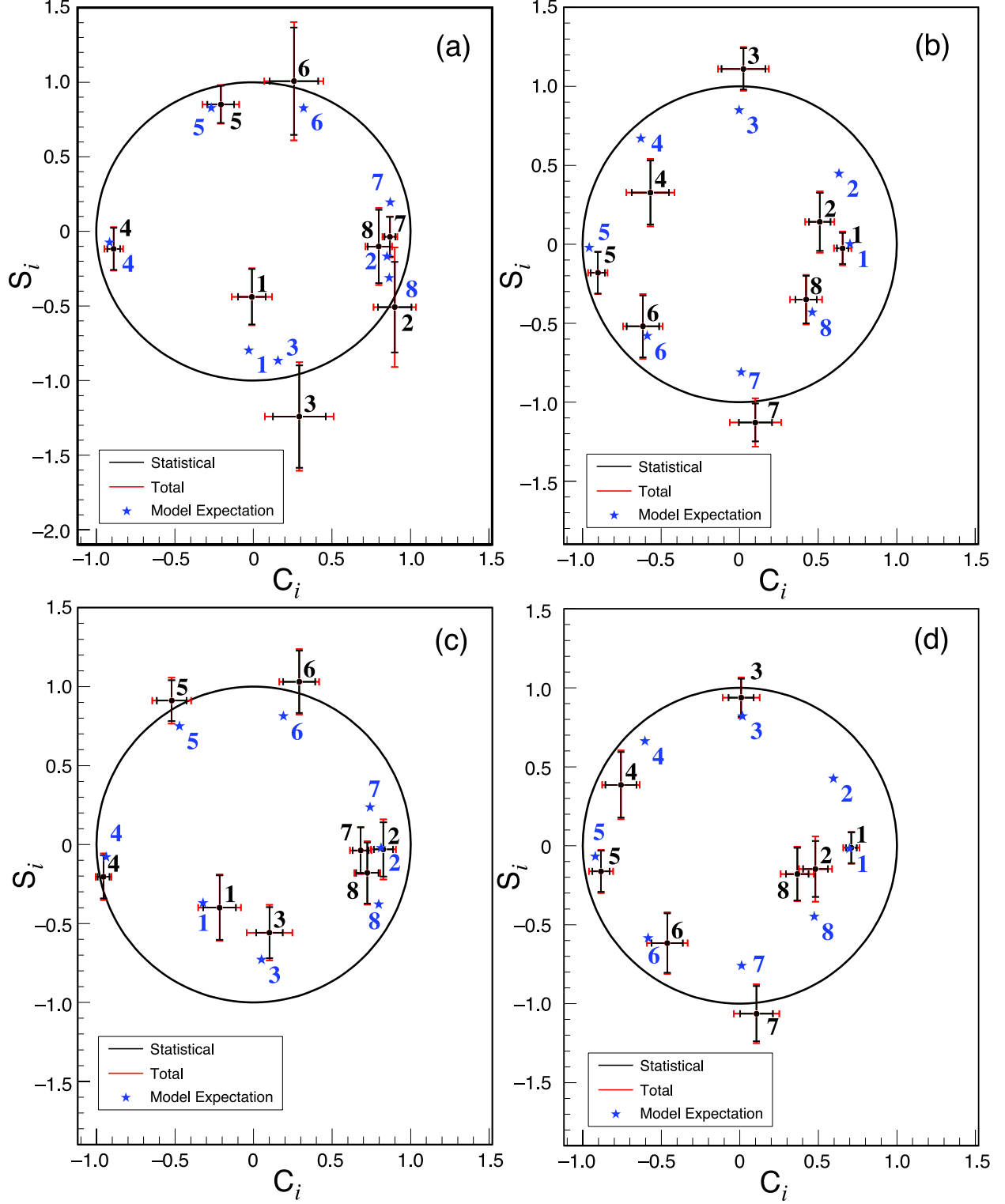
FIG. 14: Measured values of c_i and s_i for (a) the optimal binning, (b) the equal \Delta\delta_D binning, (c) the modified-optimal binning, and (d) the equal \Delta\delta_D binning based on the Belle model. The expected values calculated from the BABAR 2008 model are indicated by the stars. The circle indicates the boundary of the physical region c_i^2 + s_i^2 = 1 .
