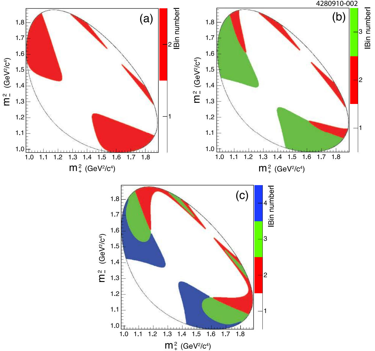
FIG. 2: Equal \Delta\delta_D division of the D^0 \rightarrow K_S^0 K^+ K^- Dalitz plot into (a) \mathcal{N} = 2 , (b) \mathcal{N} = 3 , and (c) \mathcal{N} = 4 bins.
