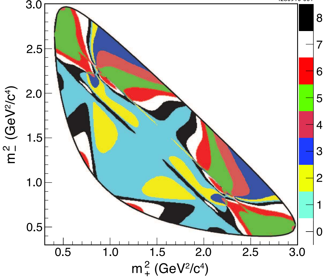
FIG. 1: Equal \Delta\delta_D binning of the D^0 \rightarrow K_S^0 \pi^+ \pi^- Dalitz plot with \mathcal{N} = 8 based on the model from Ref. [12]. The color scale represents the absolute value of the bin number, |i| .
