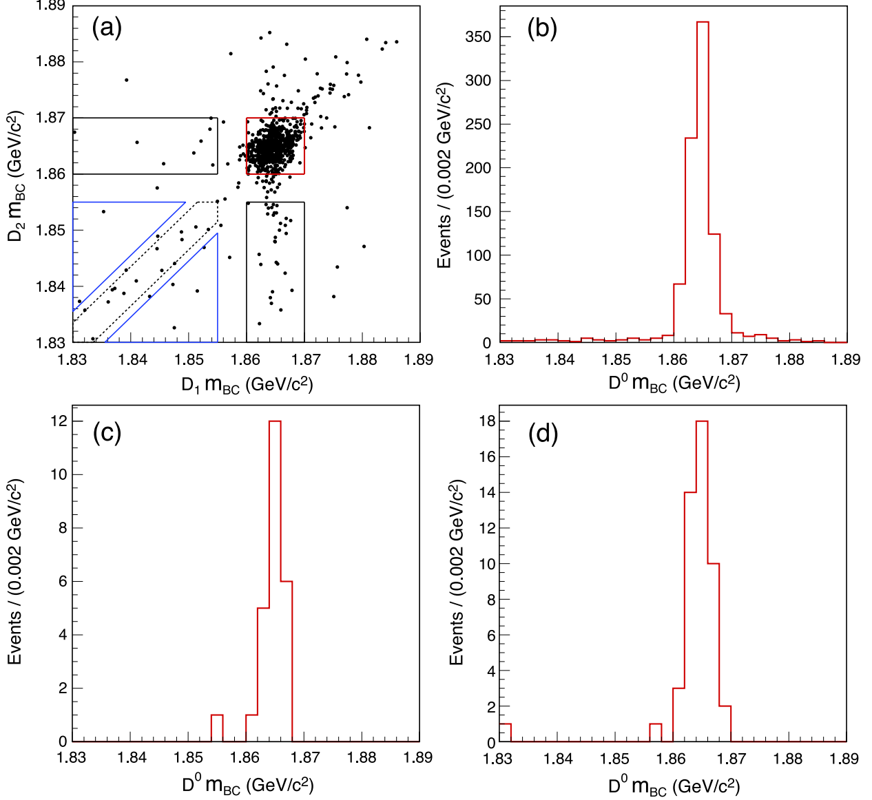
FIG. 6: (a) Distribution of m_{bc} for D^0 \rightarrow K_S^0 K^+ K^- candidates ( D_1 ) against the m_{bc} for flavor-tag candidates ( D_2 ): \bar{D}^0 \rightarrow K^+ \pi^- , K^+ \pi^- \pi^0 and K^+ \pi^- \pi^- \pi^+ . The square signal region (red online) and four sideband regions are shown. Distributions of m_{bc} for D^0 \rightarrow K_S^0 K^+ K^- candidates tagged by (b) flavor, (c) CP -even, and (d) CP -odd decays.
