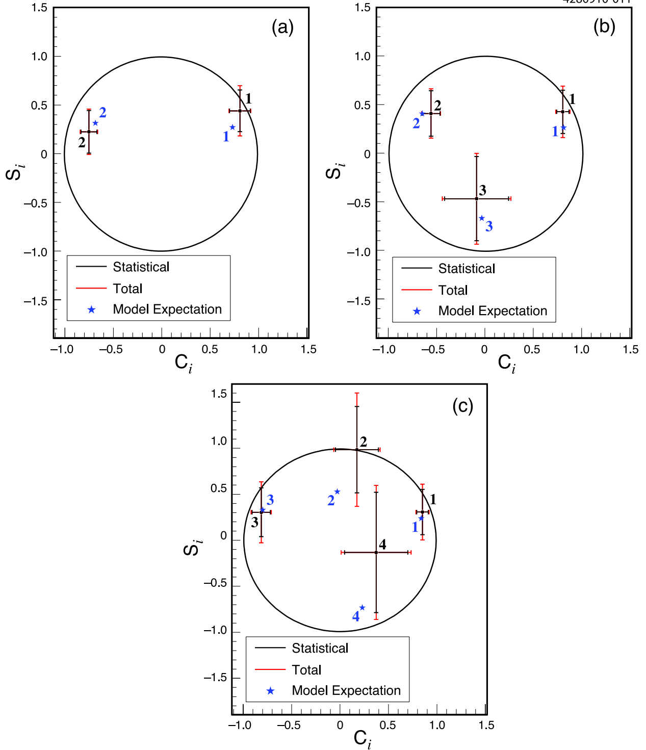
FIG. 13: Measured values of c_i and s_i for D^0 \rightarrow K_S^0 K^+ K^- data divided into (a) \mathcal{N} = 2 , (b) \mathcal{N} = 3 , and (c) \mathcal{N} = 4 equal \Delta\delta_D bins. The expected values calculated from the BABAR 2010 model are indicated by the stars. The circle indicates the boundary of the physical region c_i^2 + s_i^2 = 1 .
