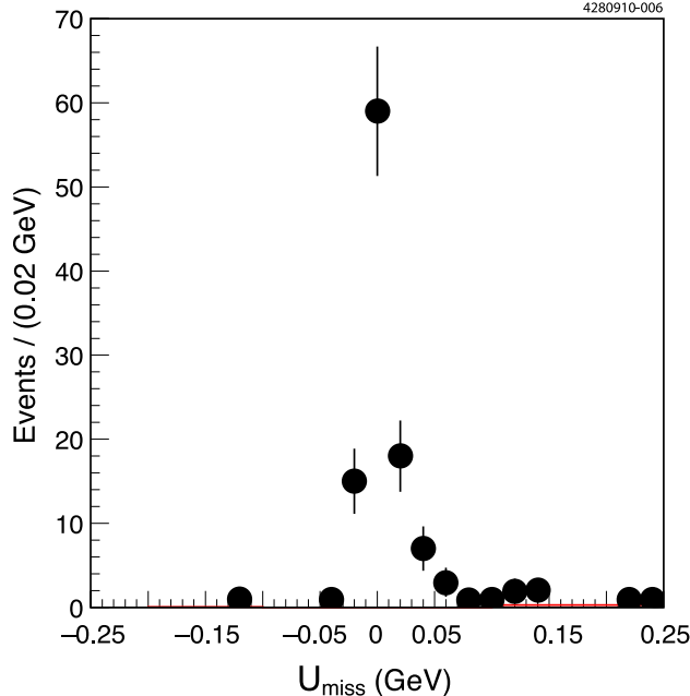
FIG. 8: U_{miss} distribution for K^+e^-\nu -tagged K_S^0K^+K^- candidates. The points are data and the solid histogram is the background estimated from simulation. The background histogram (red online) is barely visible indicating that the background is negligible.
