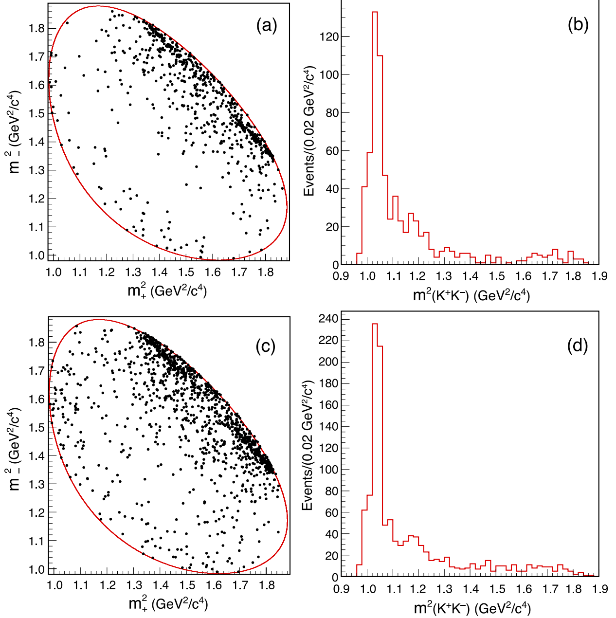
FIG. 12: (a) Dalitz plot and (b) m_{K^+K^-}^2 distributions of flavor-tagged D^0 \rightarrow K_S^0 K^+ K^- candidates. (c) Dalitz plot and (d) m_{K^+K^-}^2 distributions of flavor-tagged D^0 \rightarrow K_L^0 K^+ K^- candidates.
