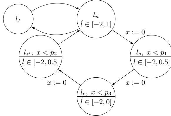
Figure 4: \mathcal{A}_H in the hypervisor modeling the pipeline failure.
