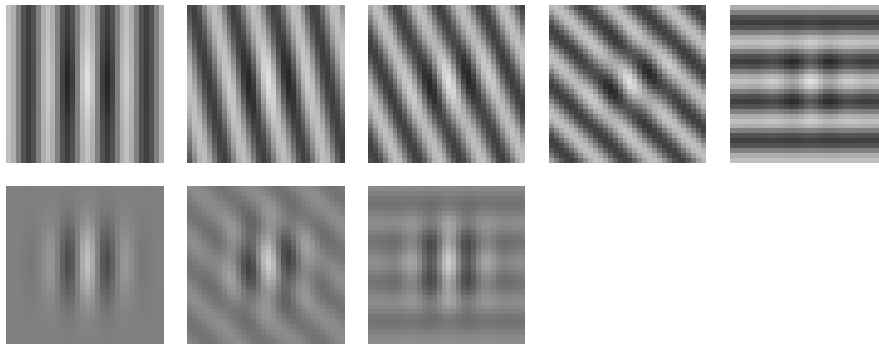
Figure 12. Stimuli of Foley and Boynton. The first row shows a Gabor target added to cosine masks at orientations of 0°, 11.25°, 22.5, 45° and 90°. Second row shows the same Gabor target added to an identical Gabor mask or a Gabor mask plus a cosine mask at 45° or 90°.
