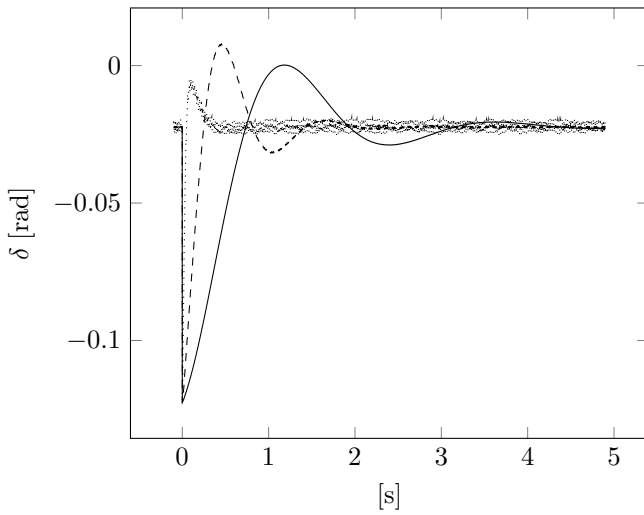
Fig. 14. Experiments. Time evolutions of the angle difference \delta , for m_a = 5 \cdot 10^{-4} (solid line), m_a = 5 \cdot 10^{-3} (dashed line) and m_a = 5 \cdot 10^{-2} (dotted line) when the angle of the inverter b is subject to an additive step disturbance of 0.1 rad.
