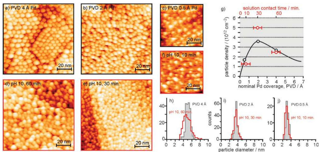
Fig. 4 STM images of Pd particles formed on \text{Fe}_3\text{O}_4(111) after deposition of various amounts of Pd by physical vapor deposition (PVD) in UHV (a–c), and after interaction with Pd precursor solution for various contact times (d–f). (The nominal Pd loading was (a) 4 Å Pd, (b) 2 Å Pd, (c) 0.5 Å Pd, and the precursor interaction times were (d) 60 min, (e) 30 min, and (f) 10 min.) (g) Pd particle density for the various preparations (black: PVD; red: precursor solution; red error bars indicate that Pd loadings obtained after various solution interaction times correspond approximately to the nominal Pd coverage in Å indicated in the bottom horizontal axis). (h), (i) and (j) represent the particle size distributions of samples (PVD 4 Å/precursor 60 min), (PVD 2 Å/precursor 30 min) and (PVD 0.5 Å/precursor 10 min), respectively. All samples were annealed to 600 K prior to STM imaging. Image size: (a), (b), (d), (e): 100 nm \times 100 nm; (c), (f): 60 nm \times 60 nm.
