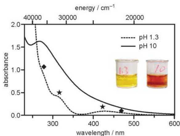
Fig. 2 UV-Vis spectra of a \text{PdCl}_2 solution in acidic (pH 1.3, dashed line) and alkaline (pH 10, solid line) medium. Symbols ♦ and ★ indicate the positions of d-d and charge transfer transitions of \text{PdCl}_4^{2-} (♦) and [\text{PdCl}_3(\text{H}_2\text{O})]^- (★) complexes in acidic solution.
