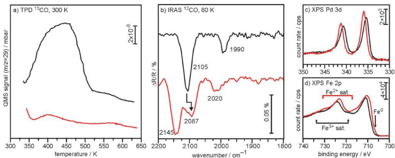
Fig. 6 Spectroscopic characterization of the Pd/Fe 3 O 4 (111) model catalyst prepared by impregnation with pH 10 Pd 2+ solution after oxidation and subsequent reduction in CO (black curves) or H 2 (red curves). (a) 13 CO TPD, (b) 12 CO IRAS, (c) Pd 3d XPS, and (d) Fe 2p XPS spectra. (The curves in a and b are vertically offset for clarity.)
