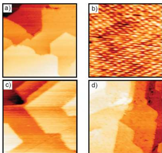
Fig. 1 STM images of freshly prepared \text{Fe}_3\text{O}_4(111) thin films. (a) Large scale image ( 100 \text{ nm} \times 100 \text{ nm} ); (b) detail scan ( 7 \text{ nm} \times 7 \text{ nm} ) showing atomic periodicity resulting from the Fe within the surface layer. (c) \text{Fe}_3\text{O}_4(111) after contact with pH 12 (NaOH) solution ( 100 \text{ nm} \times 100 \text{ nm} ). (d) After heating the surface in (c) to 600 K in UHV ( 100 \text{ nm} \times 100 \text{ nm} ).
