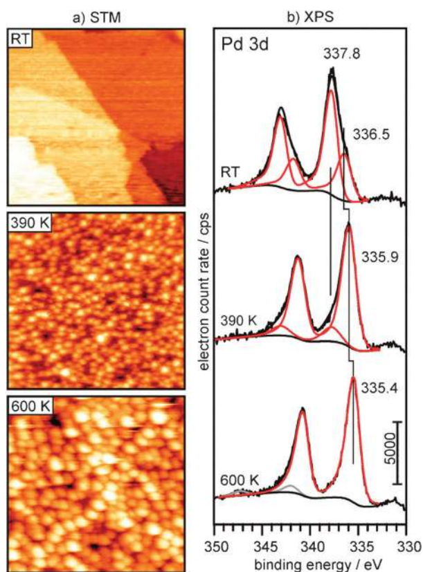
Fig. 3 (a) STM images (100 nm × 100 nm) and (b) XP spectra obtained after exposure of Fe 3 O 4 (111) to pH 10 Pd 2+ precursor solution (RT, top) and subsequent annealing to 390 K (middle) and 600 K (bottom). Fits of the individual Pd 3d XPS components are shown as red lines and the respective Pd 3d 5/2 binding energy values are reported. The two peaks shown as grey lines in the 600 K XPS spectrum result from Plasmon excitation in the metallic Pd particles.
