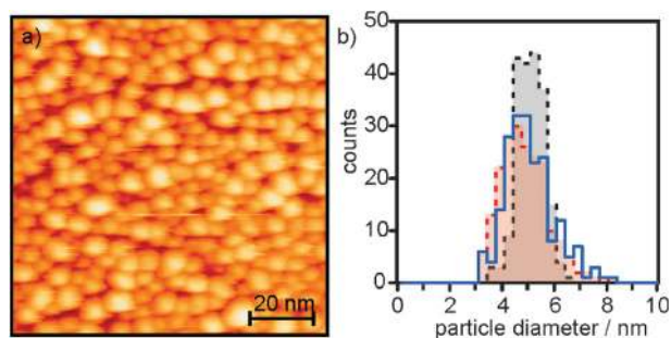
Fig. 5 (a) STM image (100 nm × 100 nm) of PVD Pd on Fe 3 O 4 (111), which had been chemically modified by exposure to pH 12 NaOH solution prior to Pd exposure. The sample was heated to 600 K in UHV prior to STM imaging. (b) Particle size distribution of Pd particles formed by PVD on clean Fe 3 O 4 (111) (black), interaction with Pd precursor solution for 60 min (red), and PVD of Pd on the chemically modified film used in (a), (blue).
