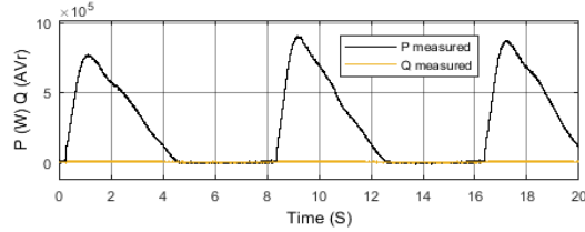
(c) Active power P (W) and reactive power Q (Var) of the PMSG
