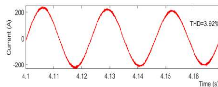
(g) Stator current i_a
