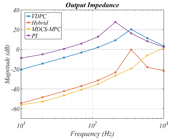
Fig. 10. Output impedance comparisons for PI [33], VDPC scheme [22], hybrid controller [24] and proposed MDCS-MPC.
