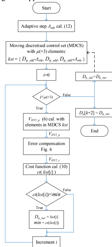
Fig. 8. The flow chat of the proposed MDCS-MPC.
