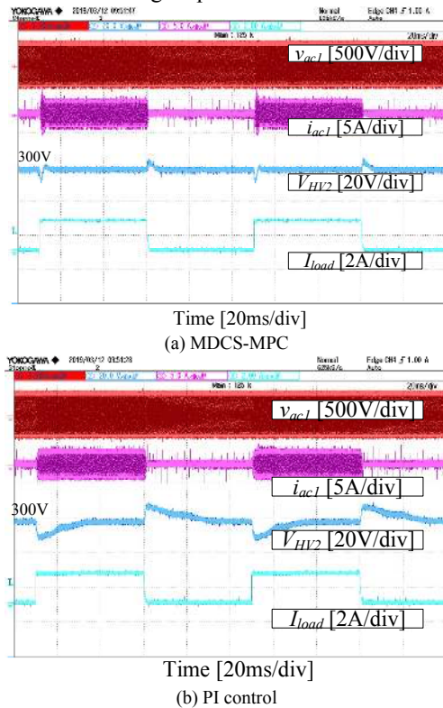
Fig. 20. Comparison between (a) proposed MDSCS-MPC, (b) PI control when the DAB converter is loaded with PPLs @20Hz.
