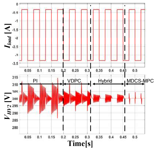
Fig. 11. Time domain load disturbance rejection ability comparison.
