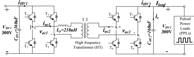
Fig. 2. The schematic of a Dual-Active-Bridge (DAB) converter.
