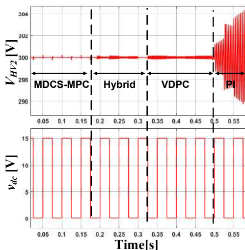
Fig. 14. Time domain source voltage disturbance rejection ability comparison.
