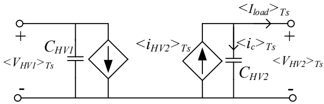
Fig. 4. The averaged model of a DAB converter [23], [24].
