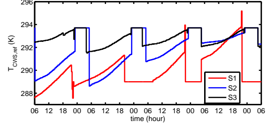
(a) Control input setpoints T_{CWS,ref}
