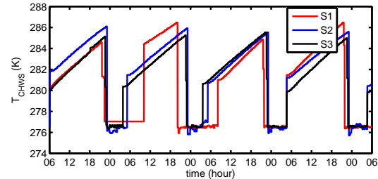
(c) Control input setpoints T_{CHWS,ref}
