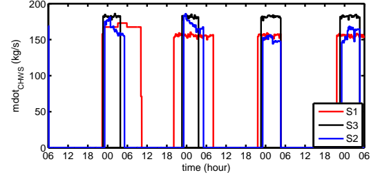
(b) Control input setpoints \dot{m}_{CHWS,ref}
