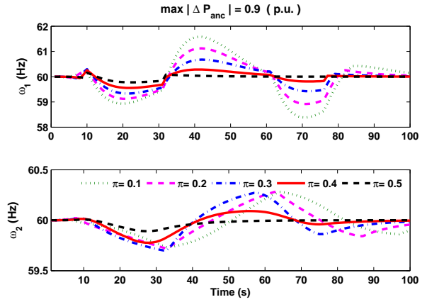
Fig. 10. Prediction horizon is H = 10 and the maximum ancillary power is \max(\Delta P_{anc}) = 0.9 (p.u.). Figure shows frequency of control areas 1 and 2. In each case, we change \max|P_{anc}| = \pi .
