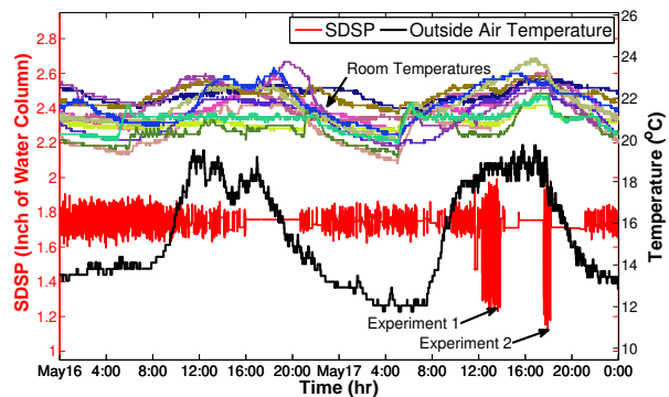
Fig. 3. SDSP set-point, outside air temperature, and temperature of 15 randomly selected rooms are shown for one day before (May 16, 2013) and the day of the experiment (May 17, 2013).
