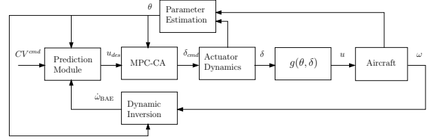
Fig. 2. RLV with MPC control allocation
