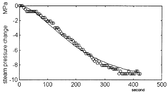
Fig. 8. Steam pressure for an increase in steam valve setting.
