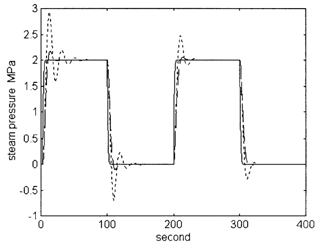
Fig. 9. Closed-loop output using linear MRAC and neurofuzzy network-based MRAC.
