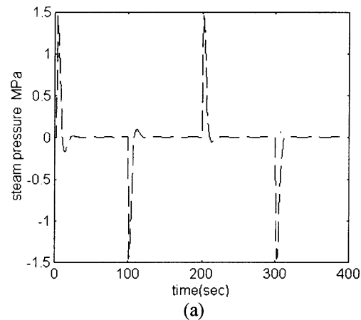
Fig. 9. Closed-loop output using linear MRAC and neurofuzzy network-based MRAC.
