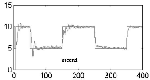
Fig. 12. Closed-loop output of nonlinear system with neurofuzzy network-based MRAC.
