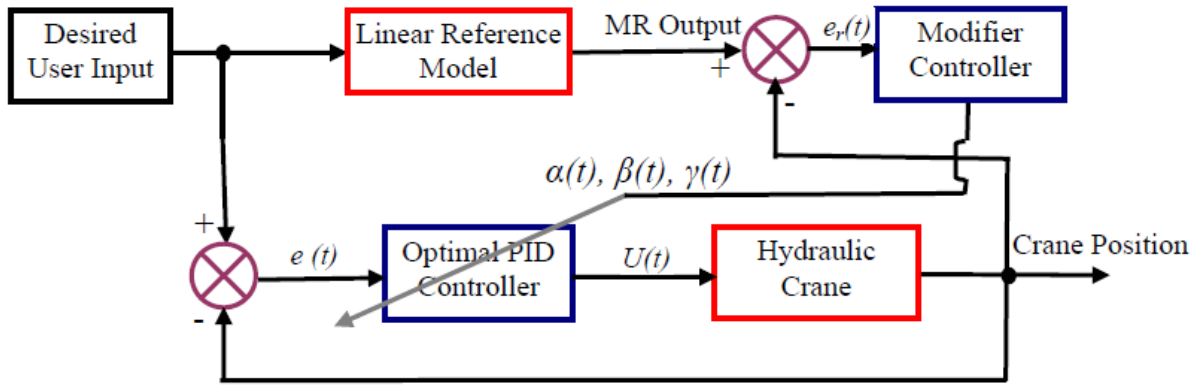
Fig. 6: Block Diagram of Crane hydraulic Control System
