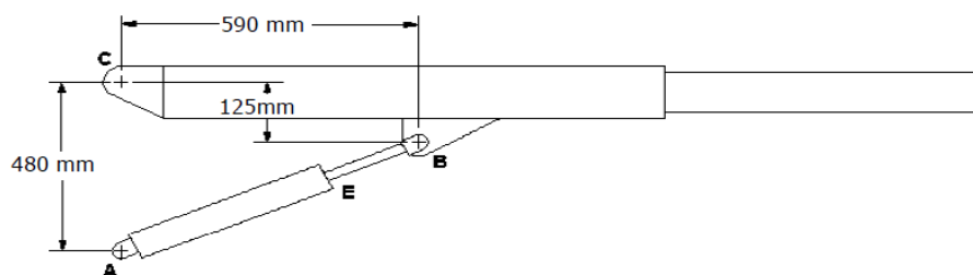
Fig. A.1: Linkage dimensions of consequence
