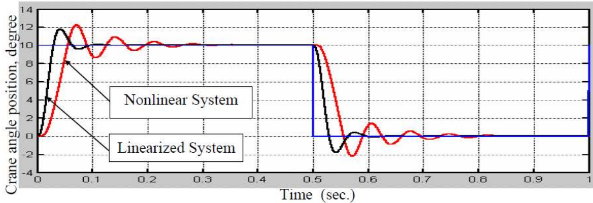
Fig. 7-a: Step response of closed loop systems with different settings
