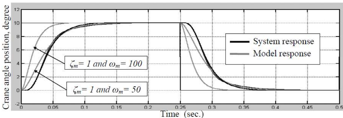
Fig. 8-a: Step response of the system based on the proposed controller
