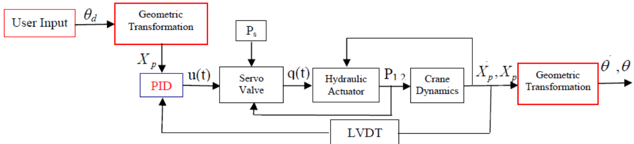
Fig. 4: Block diagram of the hydraulic crane system
