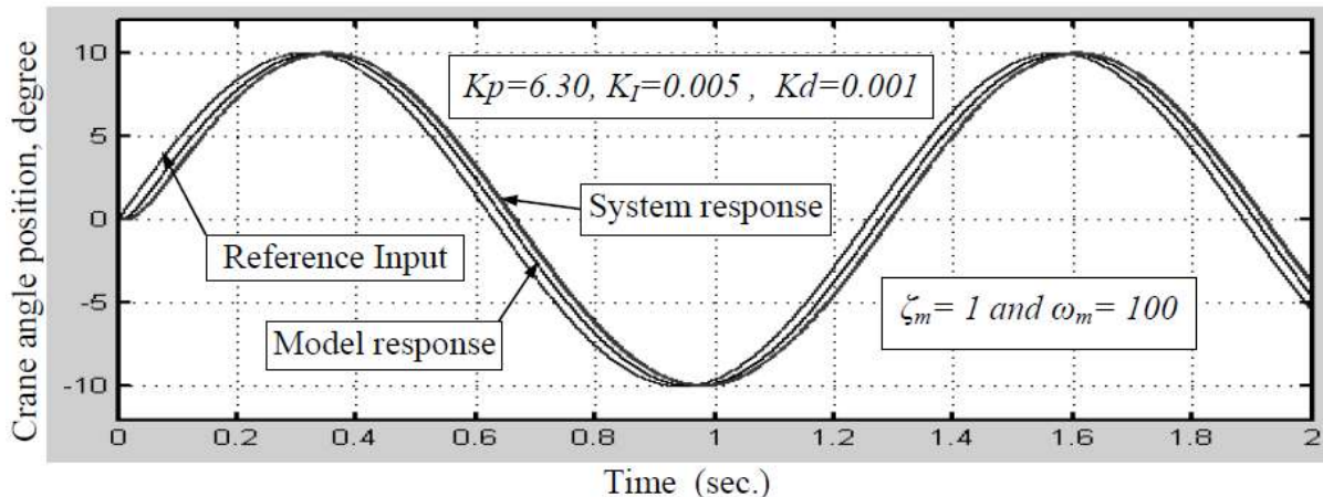
Fig. 9: Sin wave response of the system based on the proposed controller
