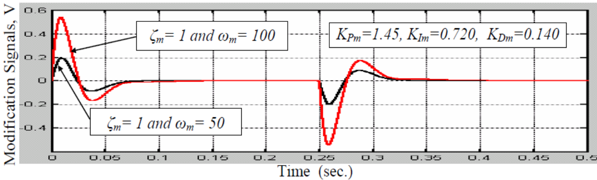
Fig. 8-c: Modifier controller signals
