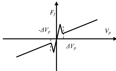
Fig.3: Characteristic of the friction
