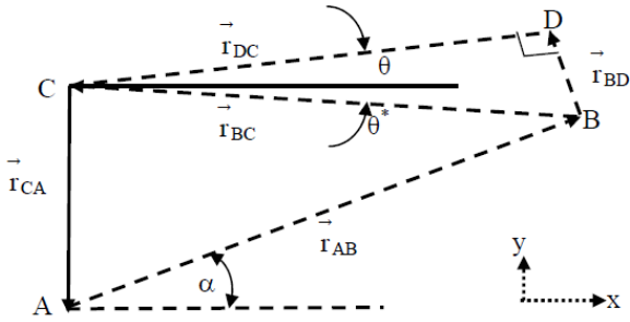
Fig. A.2: Vector representation of linkages
