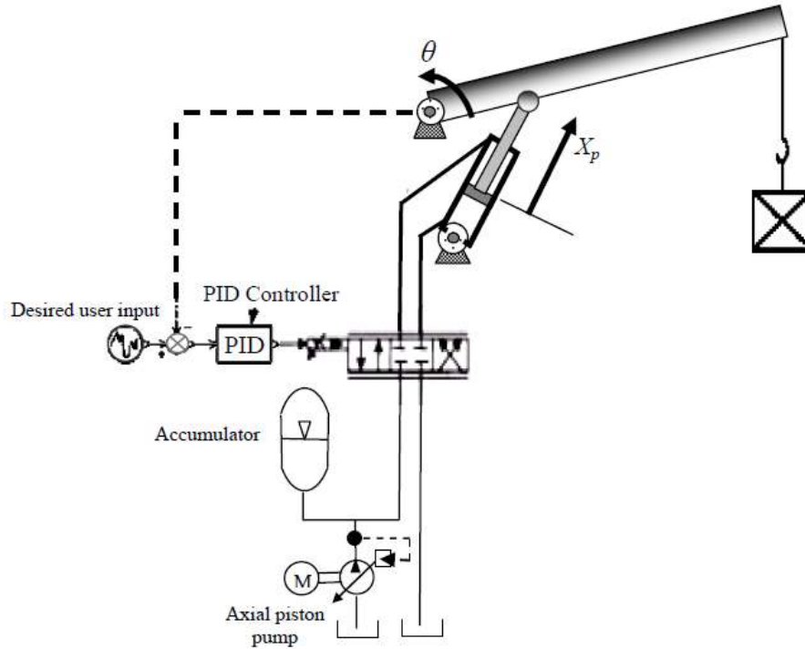
Fig. 1: Hydraulic Crane System
