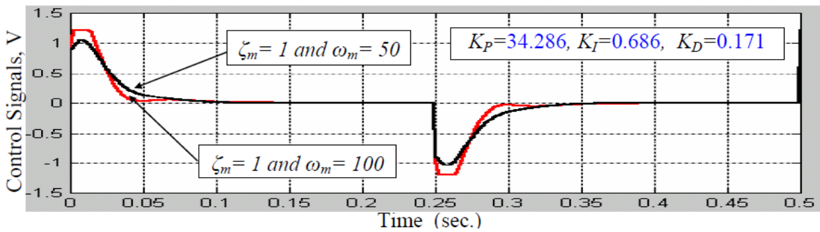
Fig. 8-b: Controller signals
