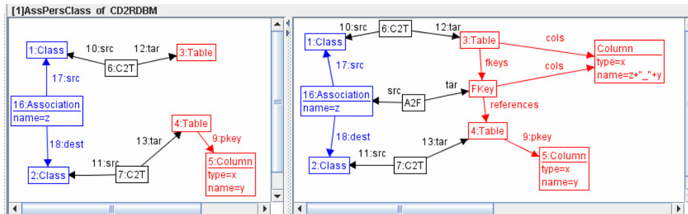
Fig. 9. Rule "AssPersClass"
