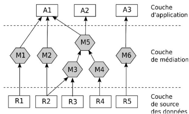
FIGURE 3.6 – Architecture de médiation
