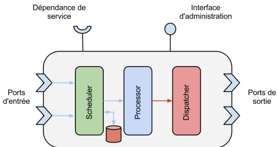
FIGURE 5.4 – Processor CILIA
