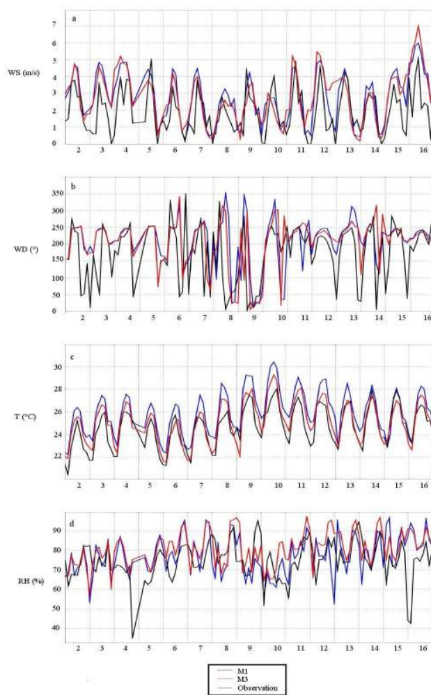
Fig. 2. Temporal variation of meteorological variables (observations and model simulations M1 and M3) from 2 to 17 July 2011; (a) wind speed ( \text{m s}^{-1} ); (b) wind direction ( ^{\circ} ); (c) air temperature ( ^{\circ}\text{C} ); (d) relative humidity (%).
