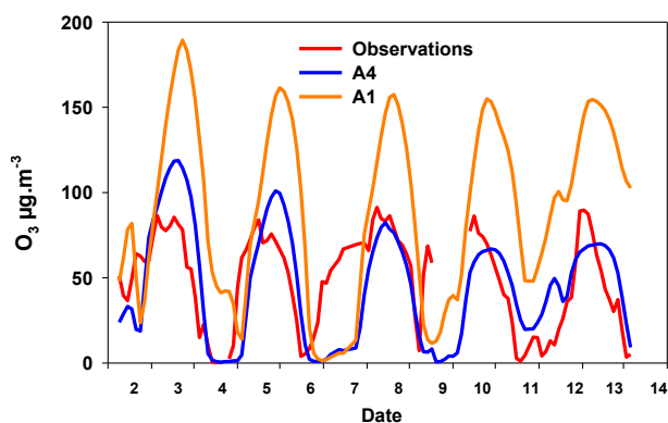
Fig. 6. Temporal variation of observed and modeled O 3 concentrations in \mu\text{g m}^{-3} from 2 to 13 July 2011.
