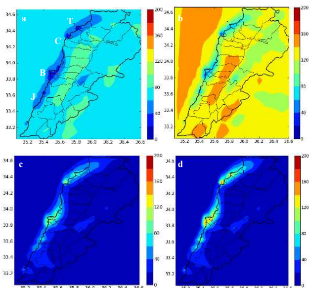
Fig. 3. Modeled average \text{O}_3 concentrations ((a) simulation A1 and (b) simulation A4) and \text{NO}_2 concentrations ((c) simulation A1 and (d) simulation A4) in \mu\text{g m}^{-3} for the outer domain D2 (T = Tripoli; C = Chekka; B = Beirut; J = Jieh).
