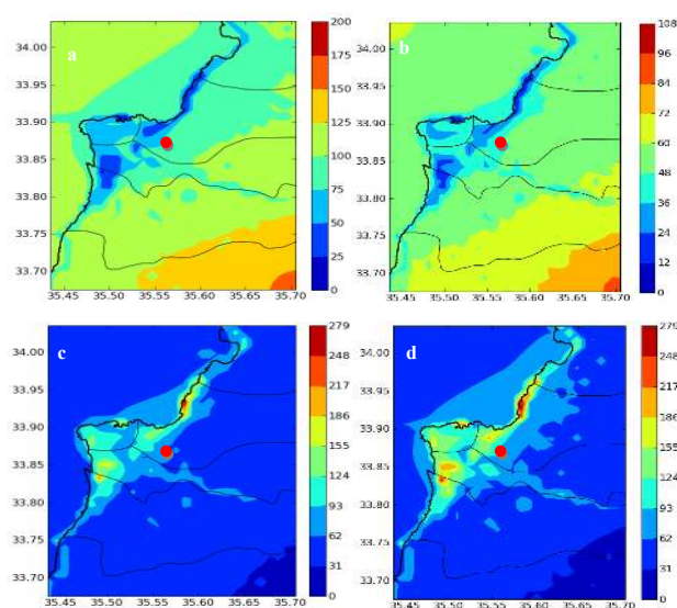
Fig. 4. Modeled average \text{O}_3 concentrations ((a) simulation A1 and (b) simulation A4) and \text{NO}_2 concentrations ((c) simulation A1 and (d) simulation A4) in \mu\text{g m}^{-3} for the inner domain D2. The red dot corresponds to the location of the measurement site at USJ during July 2011.
