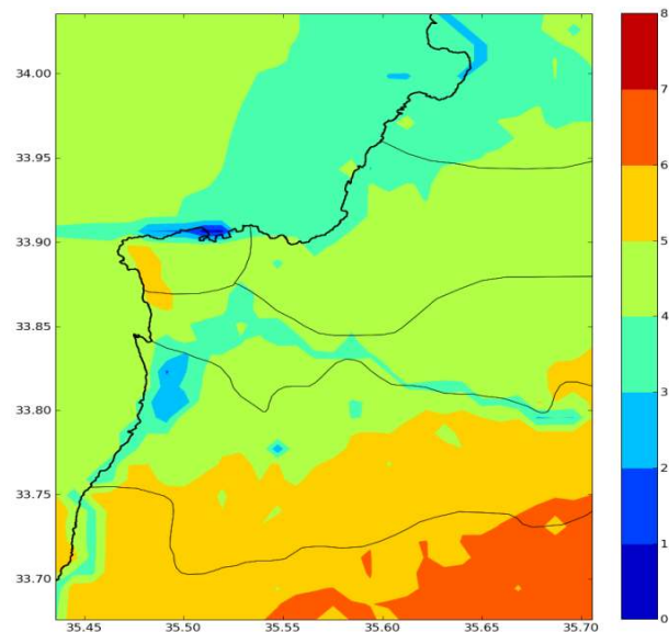
Fig. 5. Modeled average VOC/ \text{NO}_x ratio for the inner domain D1.
