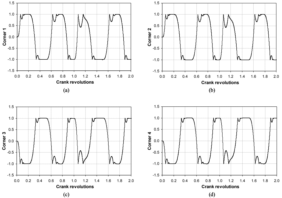
Figure 10: Dimensionless motion of the slider corners.
