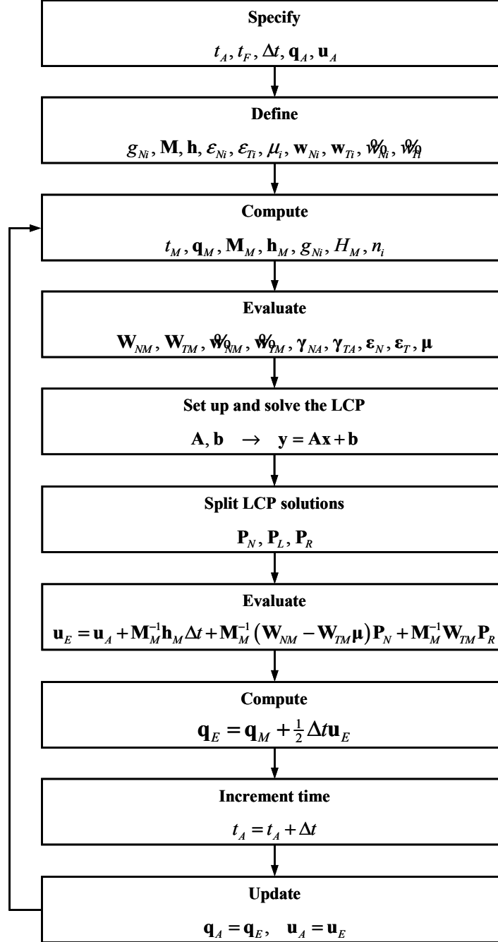
Figure 5: Flowchart of the Moreau time-stepping algorithm with an LCP formulation.
