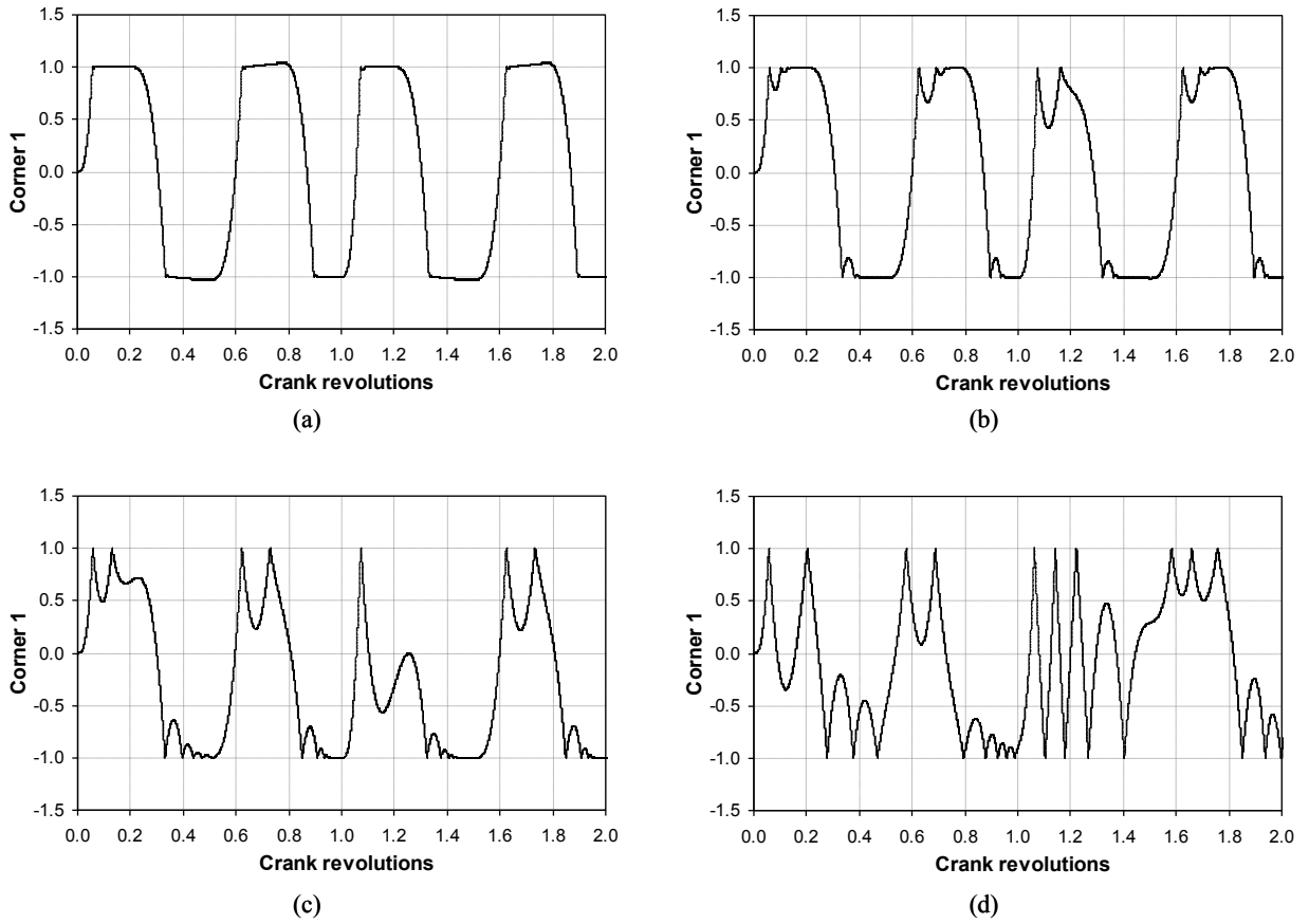
Figure 12: Influence of the restitution coefficient on the dimensionless motion of corner 1: (a) \varepsilon=0.1 ; (b) \varepsilon=0.4 ; (c) \varepsilon=0.6 ; (d) \varepsilon=0.9 .
