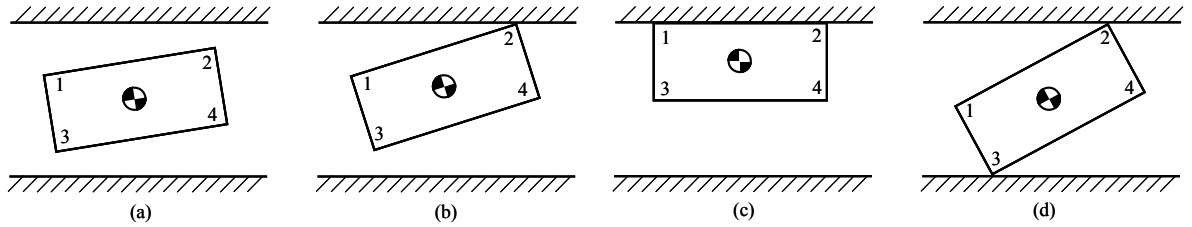
Figure 8: Different scenarios for the slider and guide interaction: (a) no contact; (b) one corner in contact with the guide; (c) two adjacent corners in contact with guide; (d) two opposite corners in contact with guide.
