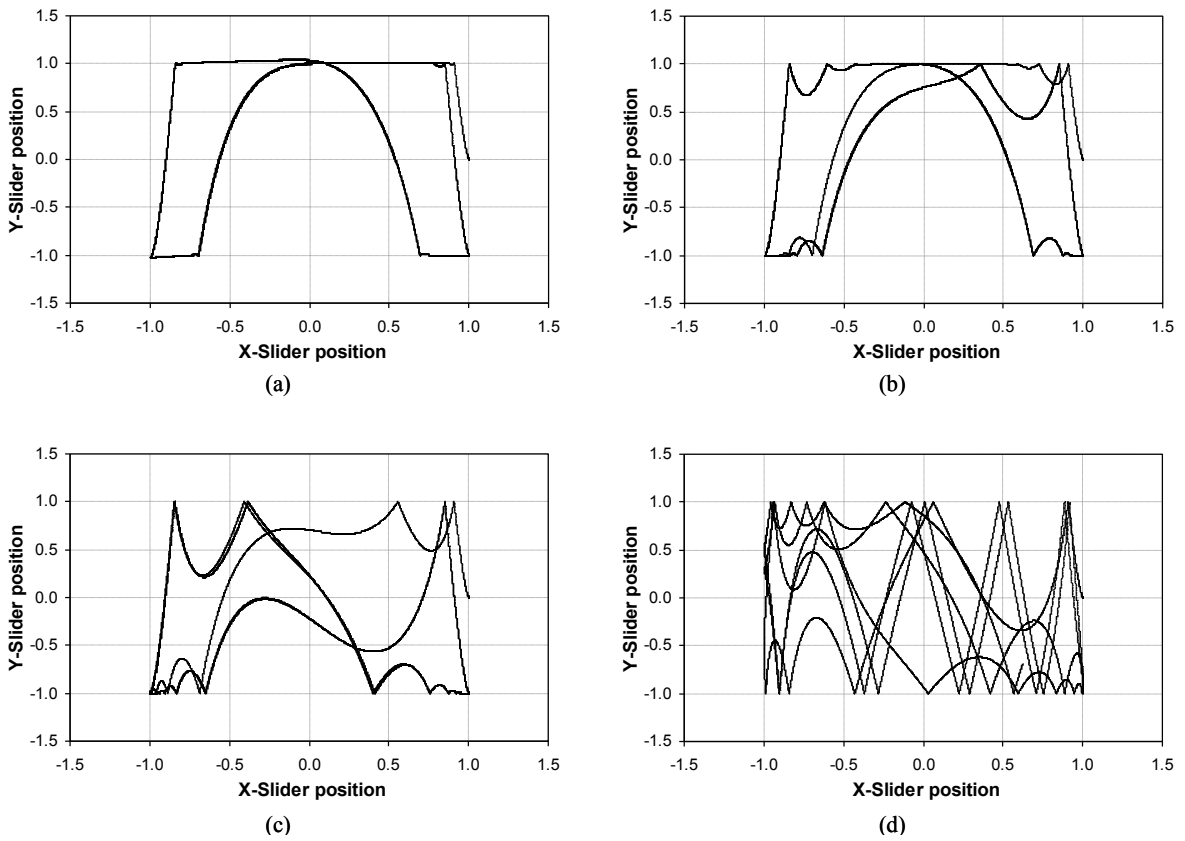
Figure 13: Influence of the restitution coefficient on the slider portraits: (a) \varepsilon=0.1 ; (b) \varepsilon=0.4 ; (c) \varepsilon=0.6 ; (d) \varepsilon=0.9 .
