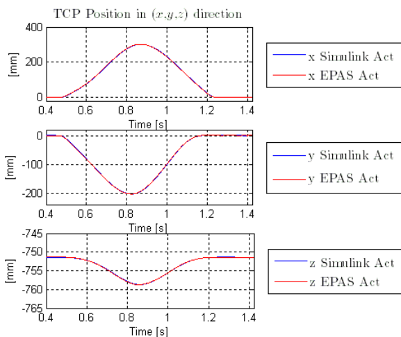
Figure 11.15, shows the TCP motion in x,y and z components of the Delta-3 robots TCP position.
