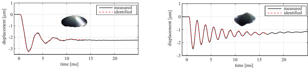
Figure 8. Measured step responses of the first and second eigenfunctions of an Alpa0 DM88 deformable membrane mirror without feedforward control showing a settling time above 5-10 ms
