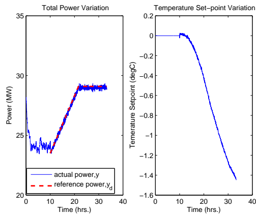
(b) Response to ramp reference and the control input
