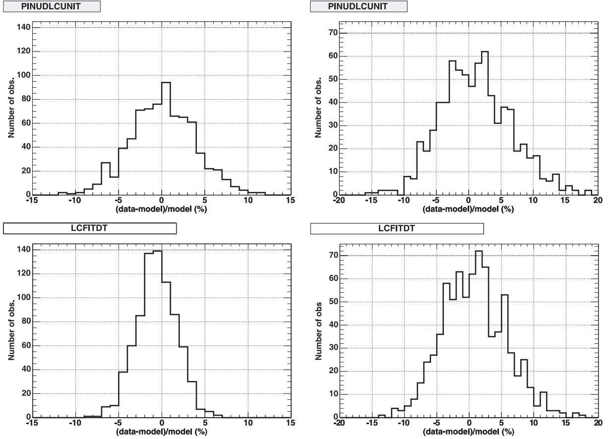
Fig. 10. Histograms of the fractional residual between the NXB data and background model. Top and bottom panels show plots for PINUDLCUNIT and LCFITDT, respectively. Left and right show plots for 15–40 keV and 40–70 keV, respectively.
