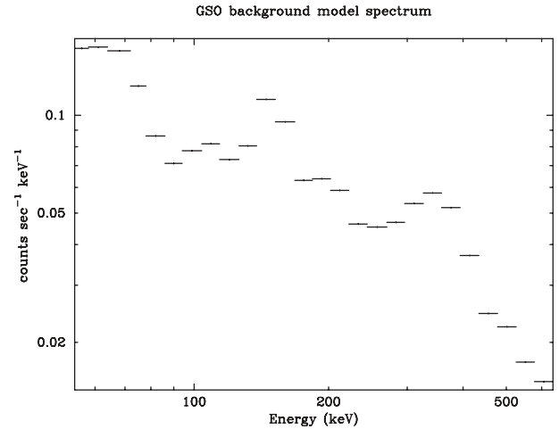
Fig. 6. Example of the GSO background model spectrum.
