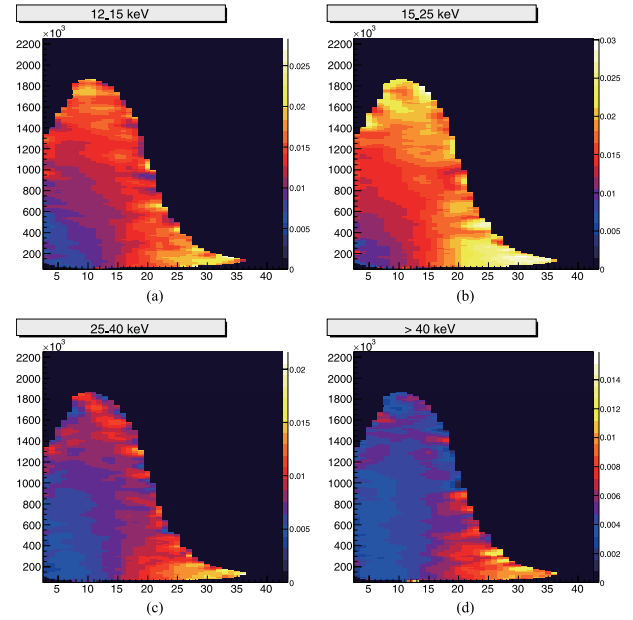
Fig. 5. NXB data base of the PINUDLCUNIT method for (a) 12–15 keV, (b) 15–25 keV, (c) 25–40 keV, and (d) > 40 keV. The horizontal and vertical axes are PINUD and PINUD_{buildup} , respectively. Color represents the count rate of the PIN NXB.
