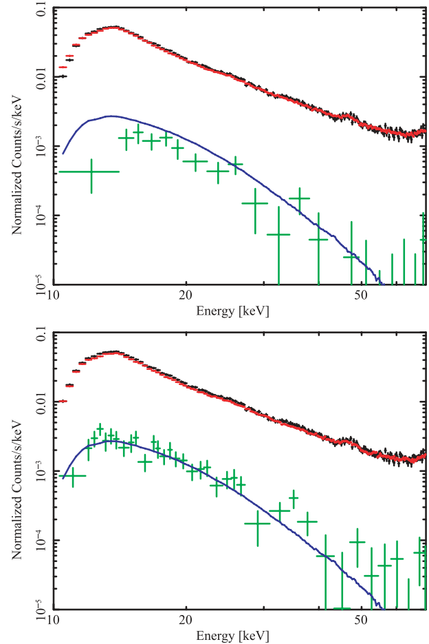
Fig. 14. Averaged spectra of sky observations (black) and the NXB model (red) of Cygnus Loop multi-pointing observations, together with the subtracted spectrum (green) and the CXB model (blue) by Boldt (1987). Top and bottom panels show plots for PINUDLCUNIT and LCFITDT, respectively.
