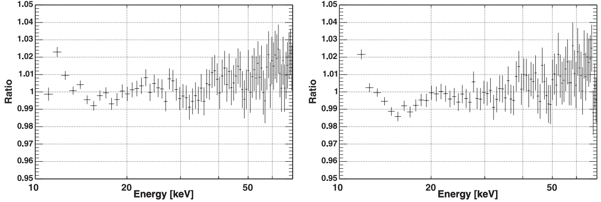
Fig. 8. Ratio of spectra between the data and the background model prediction of all available Earth occultation data (7.9 Ms exposure). Left and right panels show plots for PINUDLCUNIT and LCFITDT, respectively.
