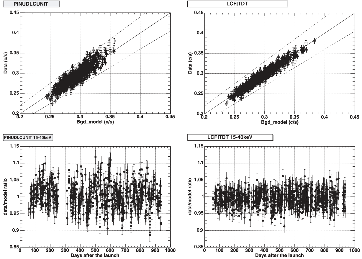
Fig. 9. Comparison of the NXB count rate in the 15–40 keV band between the data and the model prediction. Left and right panels show plots for PINUDLCUNIT and LCFITDT, respectively. Top panels show a scatter plot between the NXB data and the background model. Bottom panels show data to model the ratios of the NXB count rate, plotted against the day since 2005 July 10 (the day of Suzaku launch).
