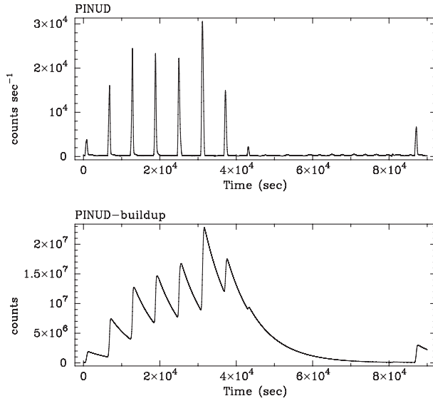
Fig. 4. Example of PINUD-buildup. The top panel shows the light curve of the PINUD count rate in units of counts s^{-1} per one unit (4 PINs), and the bottom shows the PINUD_{buildup} convolved with a time constant of 8000 s.
