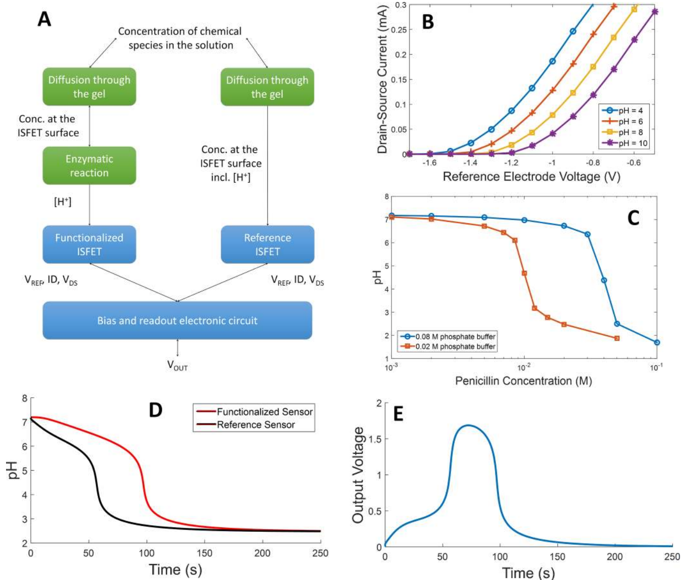
Fig 6. Results on the penicillin sensor. (A) is the overview of the building blocks of the model. Green blocks have been described in BB-SPICE whereas blue ones have been described directly in NGSPICE and integrated in the BB-SPICE netlist preceded by the \exists character. (B) is a drain-source current vs reference electrode voltage characteristics of the ISFET alone. (C) and (D) are the simulation results for the biological part of the model alone. (C) is the variation of pH in the solution as a function of concentration of penicillin for two different phosphate buffer concentrations. (D) is the transient evolution of the pH on the gate of both ISFETs for a penicillin concentration of 0.05 mol/l. Finally, (E) is a transient simulation for the whole model (biological part, ISFETs, biasing and processing electronics). The evolution of the output voltage is given for different initial penicillin concentrations.
