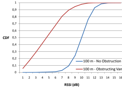
Fig. 5. Distribution of the RSSI for 100 m in case of LOS (no obstruction) and non-LOS (obstructing van) at 2.4 GHz. © [2011] IEEE
