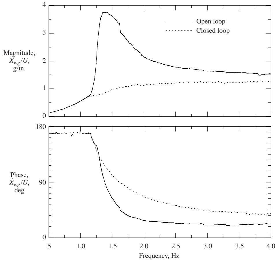
Figure 11. Upper acceleration to shaker position transfer function.
