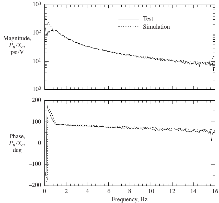
Figure 7. Upper chamber pressure to servo command transfer function.
