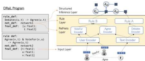
Figure 2: General overview of DRaIL.
