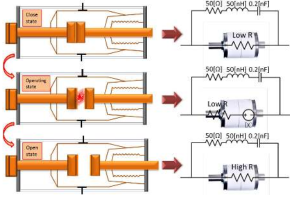
Fig. 3. VI state transitions.
