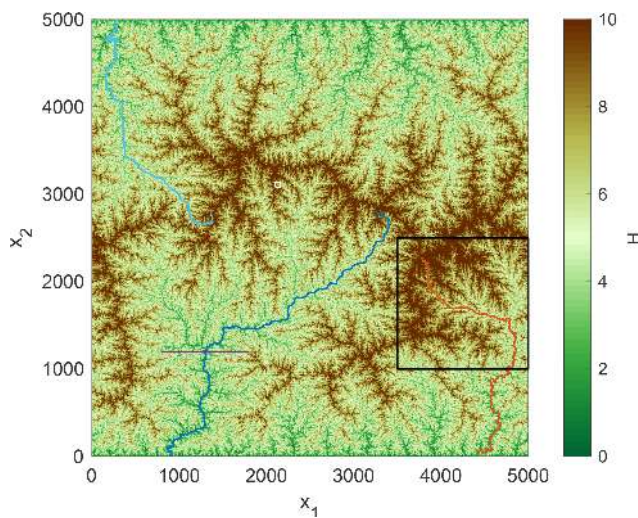
Figure 3. Fluvial equilibrium topography under uniform uplift (Hergarten, 2020, Fig. 1a). The small, white square depicts the domain of Fig. 2 and the black square the domain of Figs. 10 and 12. The blue and red lines show the three biggest rivers. The violet line refers to the profile shown in Fig. 5.
