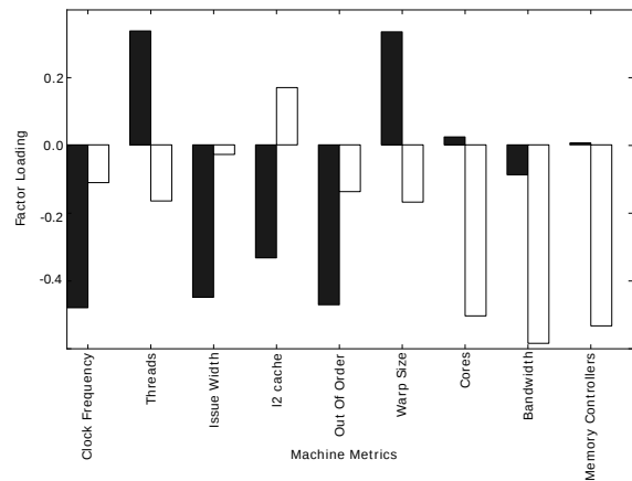
Figure 3: Factor loadings for two machine principal components. PC0 (black) corresponds to single core performance, while PC1 (white) corresponds to multi-core throughput.
