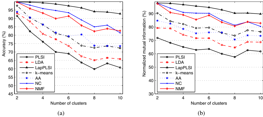
Figure 1: (a) Accuracy (b) Normalized mutual information vs. the number of classes on TDT2 corpus
