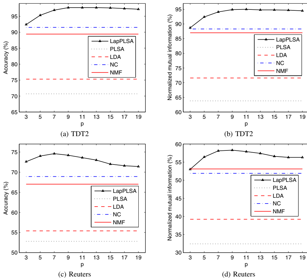
Figure 4: The performance of LapPLSI vs. parameter p . LapPLSI achieves good performance with the parameter p varying from 5 to 11.
