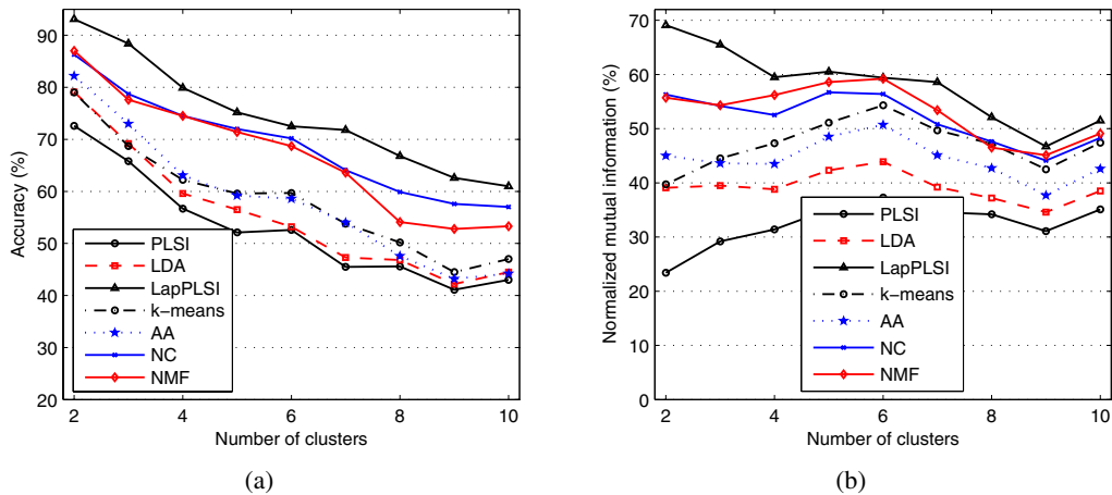
Figure 2: (a) Accuracy (b) Normalized mutual information vs. the number of clusters on Reuters corpus
