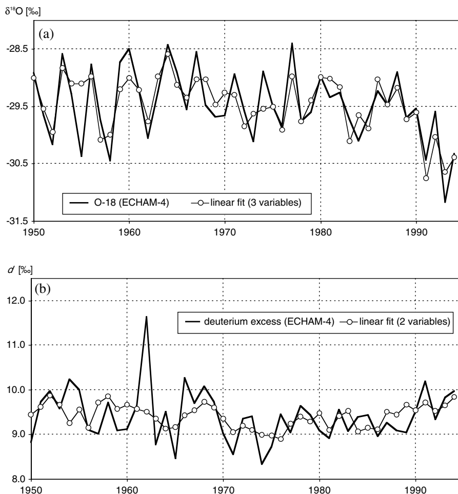
Figure 4. (a) Simulated annual \delta^{18}\text{O} record of central Greenland and the fit of a multiple linear regression (three climate variables: inversion temperature west of Greenland, sea level pressure anomalies centered over Spain, and relative humidity of mid-latitude Atlantic region) for the period 1950–1994. (b) Simulated annual deuterium excess record of central Greenland and the fit of a multiple linear regression (two climate variables: mean Atlantic SST 20^{\circ} – 40^{\circ}\text{N} and 60^{\circ} – 90^{\circ}\text{N} ).
