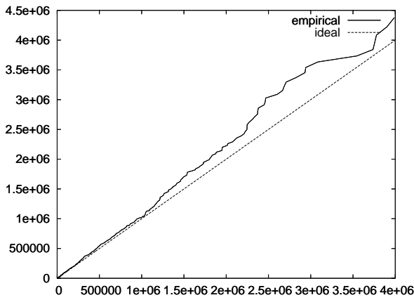
Figure 20. Q-Q Plot showing ideal case of sample drawn directly from tested Weibull distribution
