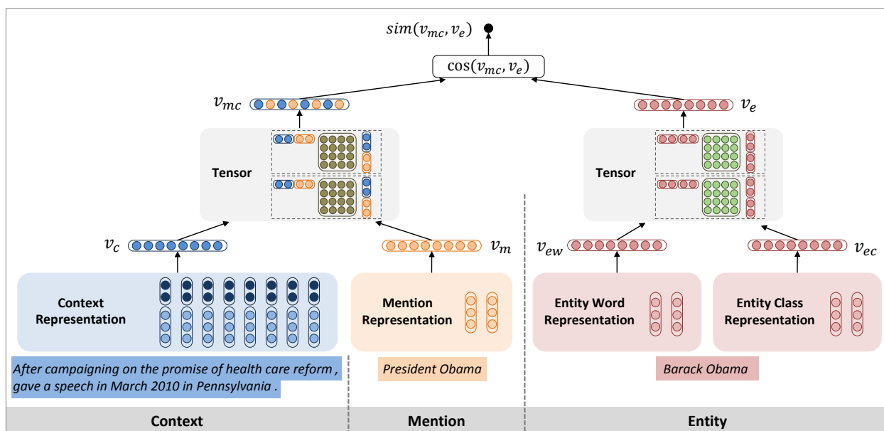
Figure 1: The proposed neural network method for entity disambiguation. In this example, the mention “ President Obama ” comes from an original document “ After campaigning on the promise of health care reform, President Obama gave a speech in March 2010 in Pennsylvania. ”. The candidate entity in this example is “ Barack Obama ”.
