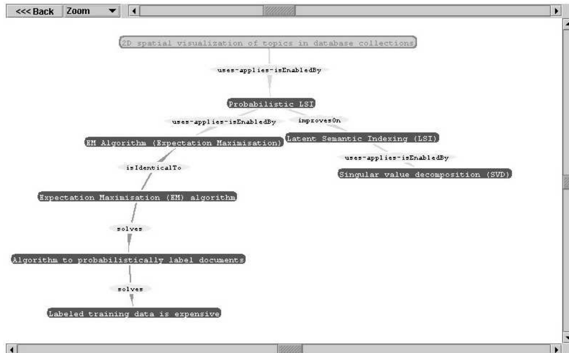
Figure 15: The Lineage service was conceived as a way to trace the ‘intellectual roots’ of a concept, displayed at the top. The network is analysed and filtered to show potentially significant relational types such as uses/applies/is enabled by , improves on , and solves . The Descendants service traverses the graph in the opposite direction to show impact of a concept.
