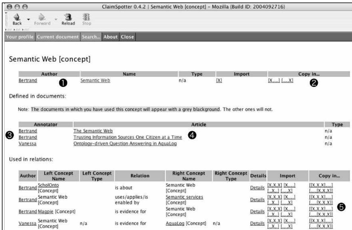
Figure 8: The user can access a History window for a Concept which displays, for instance, the author (1) and the different uses of that Concept over the corpus of documents (3) (4). It can be copied in the current document with a single click, if a user decides so (2). In a similar way, the different relations in which it is used can be imported in the document being currently annotated, or copied in order to discuss them (5). Multiple links within the History window allow a quick navigation within the annotation repository.
