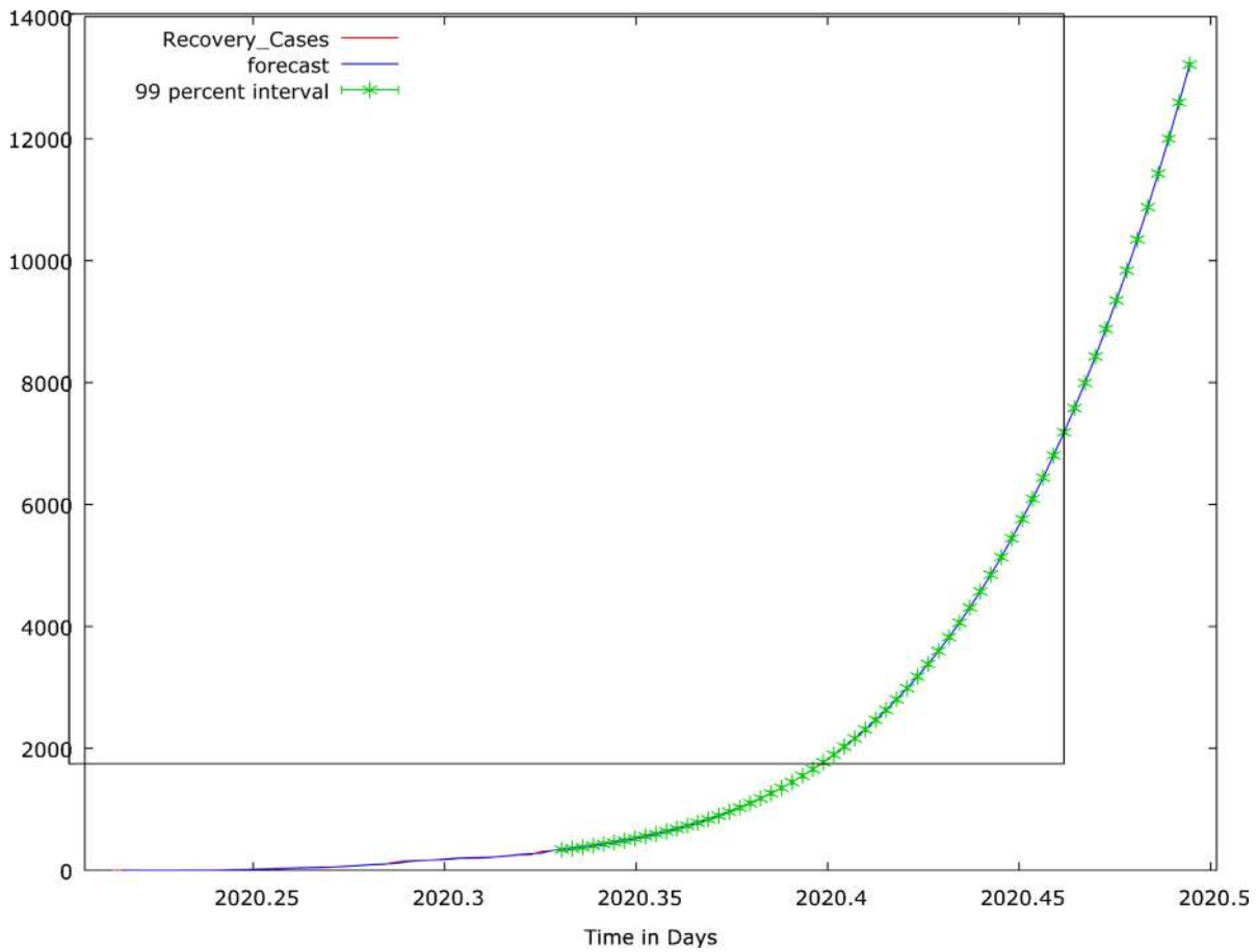
Fig. 7. COVID-19 Discharged Cases for First Sixty Four Days and its forecast values for May and June, 2020: CORC Estimator.
