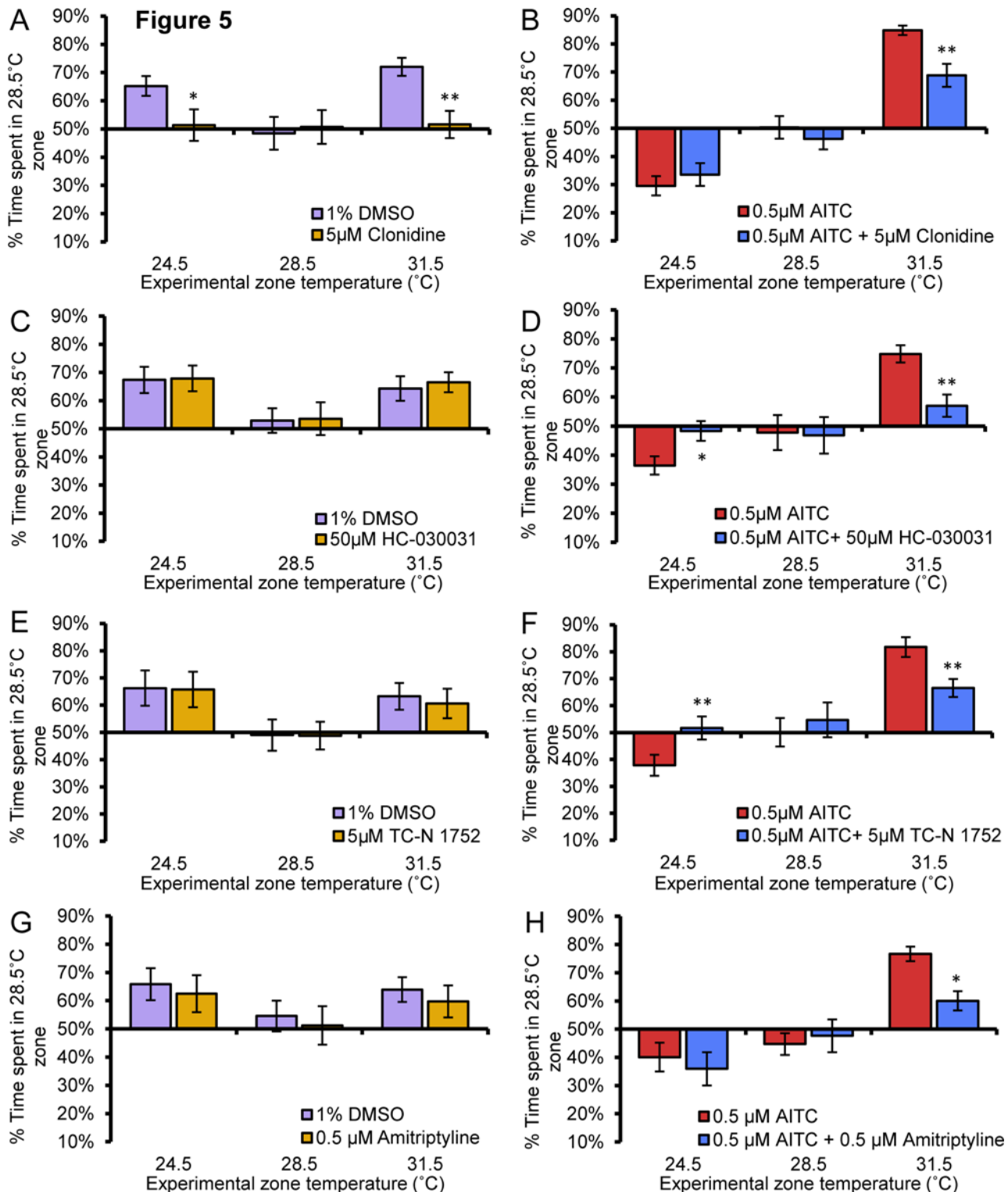
Figure 5. Analgesic molecules have differential effects on thermal aversion. A , Clonidine (5μM) significantly reduced 24.5°C and 31.5°C aversion when compared to vehicle treated larvae (2-way anova post hoc comparison) and eliminated aversion to 24.5°C and 31.5°C as measured by no significant difference from chance (1-way anova against a hypothetical mean of 50%). Clonidine did not induce aberrant zone preference (1-way anova against a hypothetical mean of 50%) and clonidine treated larvae did not differ from vehicle treated larvae in the 28.5°C vs 28.5°C assay (2-way anova post hoc comparison). B , Clonidine significantly reduced AITC sensitized aversion to 31.5°C but not 24.5°C preference when compared to vehicle treated larvae (2-way anova post hoc comparison). Clonidine did not induce aberrant zone preference (1-way anova against a hypothetical mean of 50%) and did not differ
