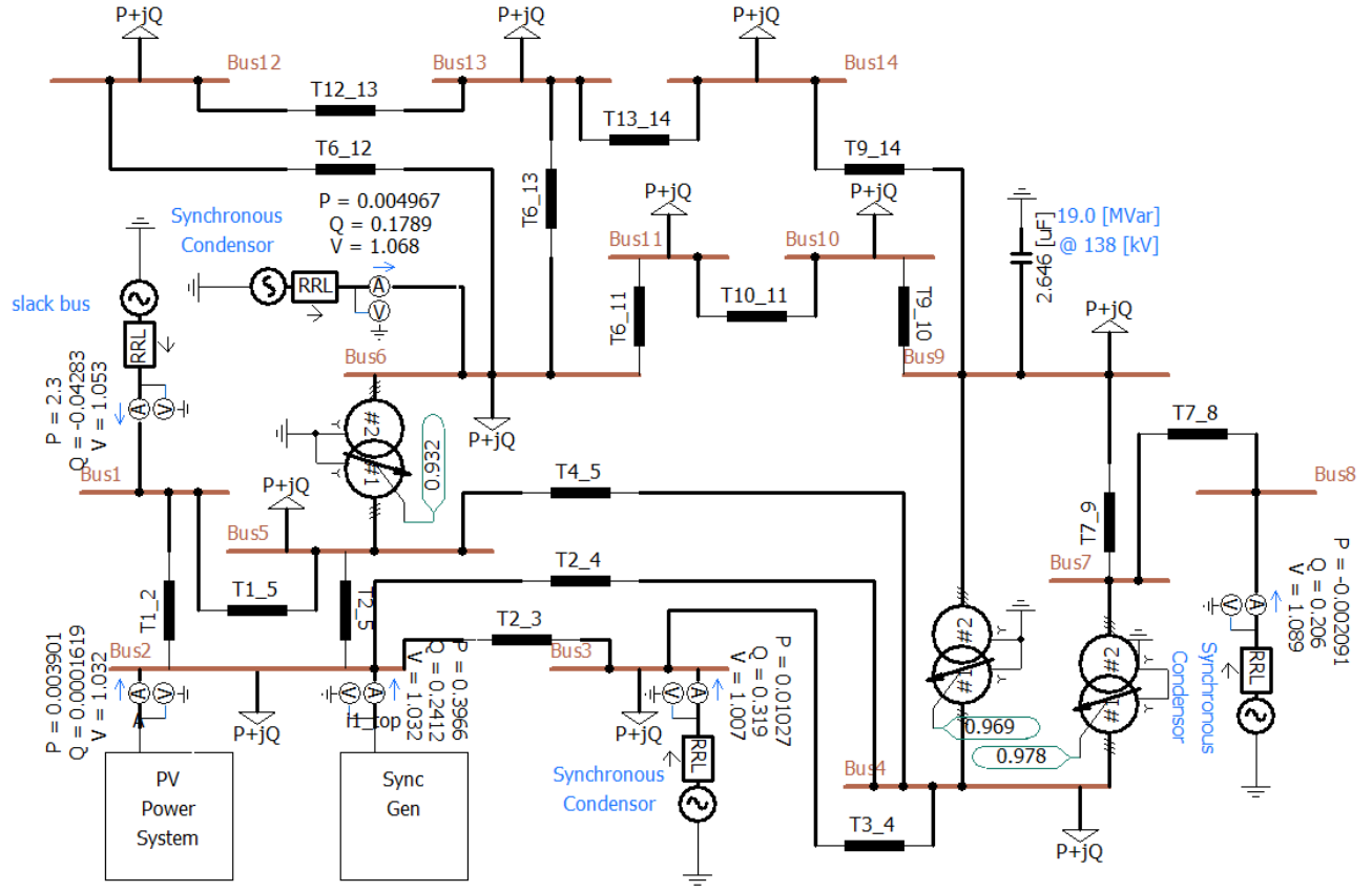
Fig. 13. Circuit diagram for the modified IEEE 14 Bus system considered in the study. The PV farm is connected to the second bus.
