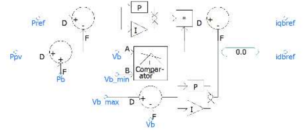
Fig. 6. Control diagram for the battery showing the voltages corresponding to maximum and minimum states of charge V_{bmax} and V_{bmin} . The d and q axes reference currents are fed to an inner current controller, or used to generate voltage references which are subsequently used to generate the gating signals (not shown).
