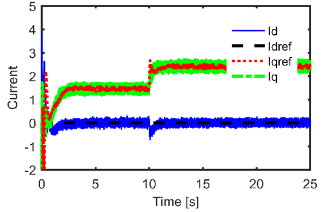
Fig. 10. The reactive, d-axis, and active, q-axis, currents are maintained at their respective references following the change in insolation. In this example, the d-axis current is maintained at zero value, and the q-axis current is determined by the power input.
