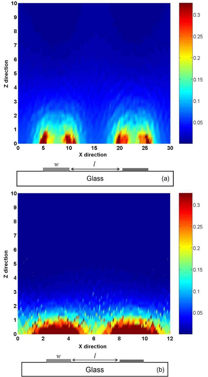
Fig. 6. Induced \Delta n profile of BPLC in a 10- \mu\text{m} IPS cells at \lambda = 550 \text{ nm} with (a) w = 5 \mu\text{m} and l = 10 \mu\text{m} at 170 V_{\text{rms}} and (b) w = 2 \mu\text{m} and l = 4 \mu\text{m} at 130 V_{\text{rms}} .
