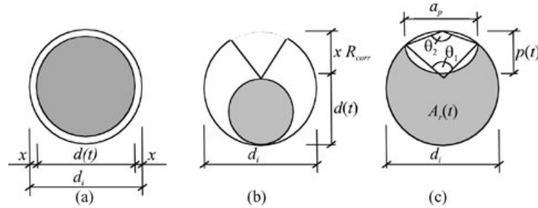
Fig. 4. The geometry of corroded steel rebar: (a) uniform corrosion (Rodriguez et al., 1996), (b) pitting corrosion (Rodriguez et al., 1996), and (c) pitting corrosion (Val and Melchers, 1998).
