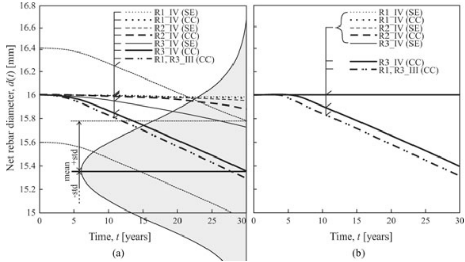
Fig. 8. The drop in rebars’ diameters over time due to corrosion for boundary conditions III and IV: (a) without and (b) with the assumption of critical chloride concentration according to Papadakis et al. (1996).
