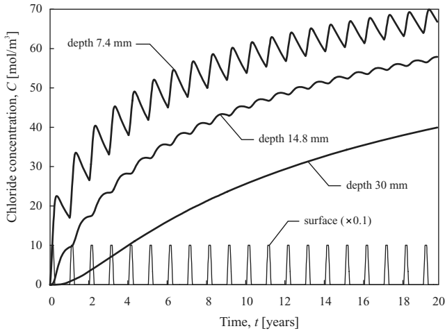
Fig. 3. The effect of seasonal de-icing salt application at different depths of concrete and the concentration on the surface (external salt feed), which is multiplied by 0.1.
