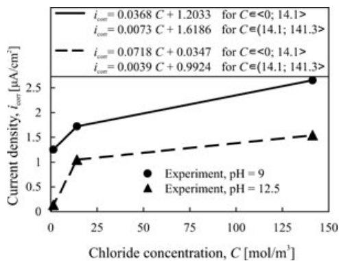
Fig. 5. The dependence of current density on chloride concentration.
