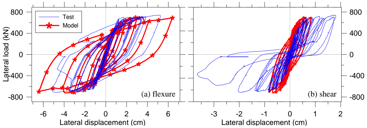
Figure 4.2. Lateral load vs. top displacement components for specimen SP 2: (a) flexure, (b) shear
