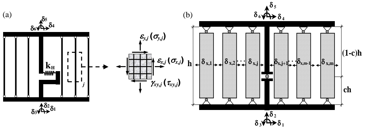
Figure 2.1. Element models: (a) original MVLEM element and (b) coupled SFI model element
