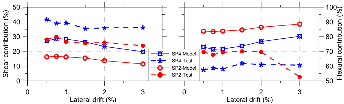
Figure 4.4. Shear and flexural components of top displacement for specimens SP 2 and SP 4: (a) shear, (b) flexure
