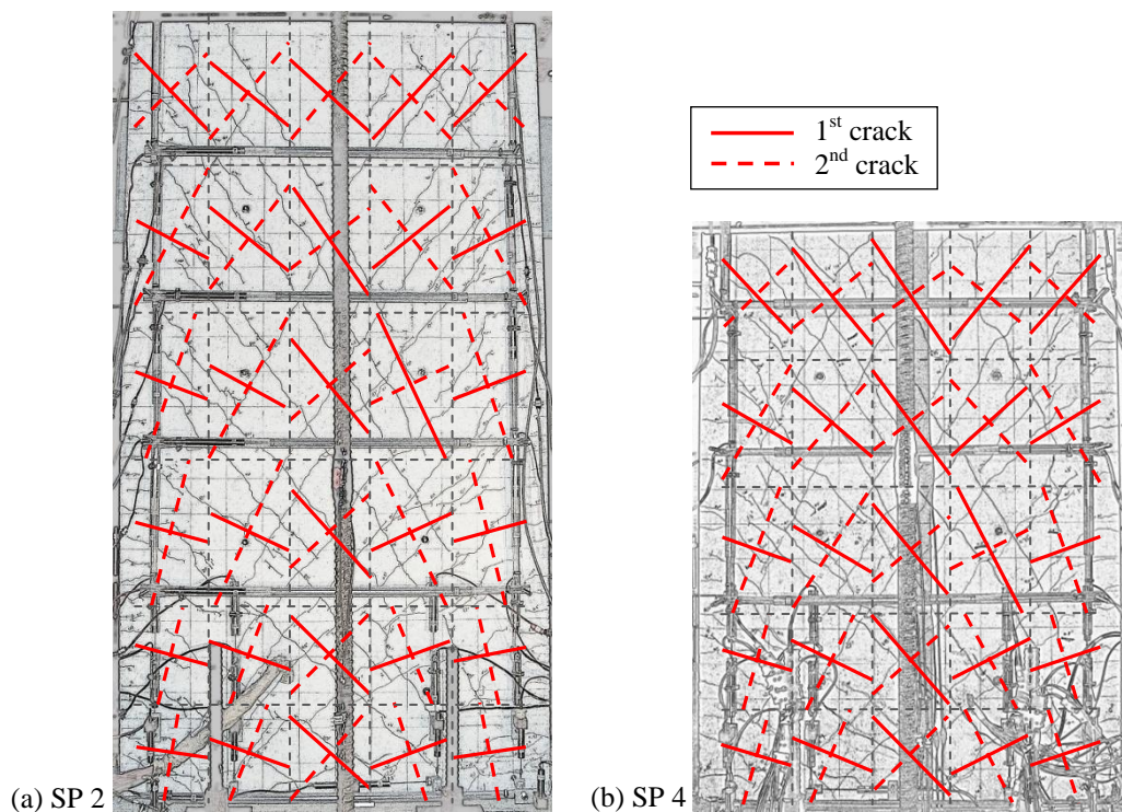
Figure 4.5. Comparison of crack patterns and model discretization: (a) specimen SP 2, (b) specimen SP 4
