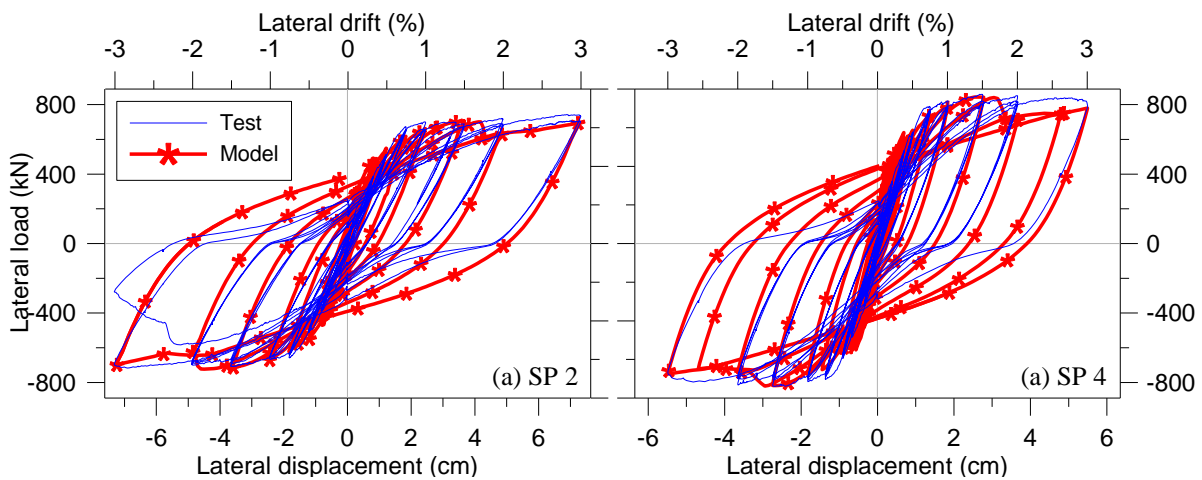
Figure 4.1. Lateral load vs. wall top displacement: (a) specimen SP 2, and (b) specimen SP 4
