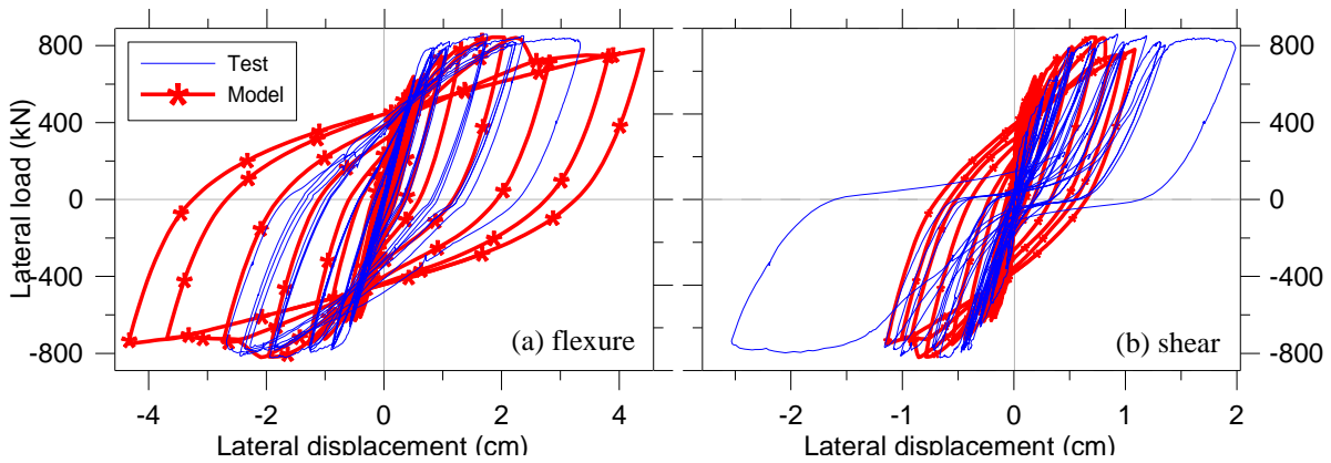
Figure 4.3. Lateral load vs. top displacement components for specimen SP 4: (a) flexure, (b) shear
