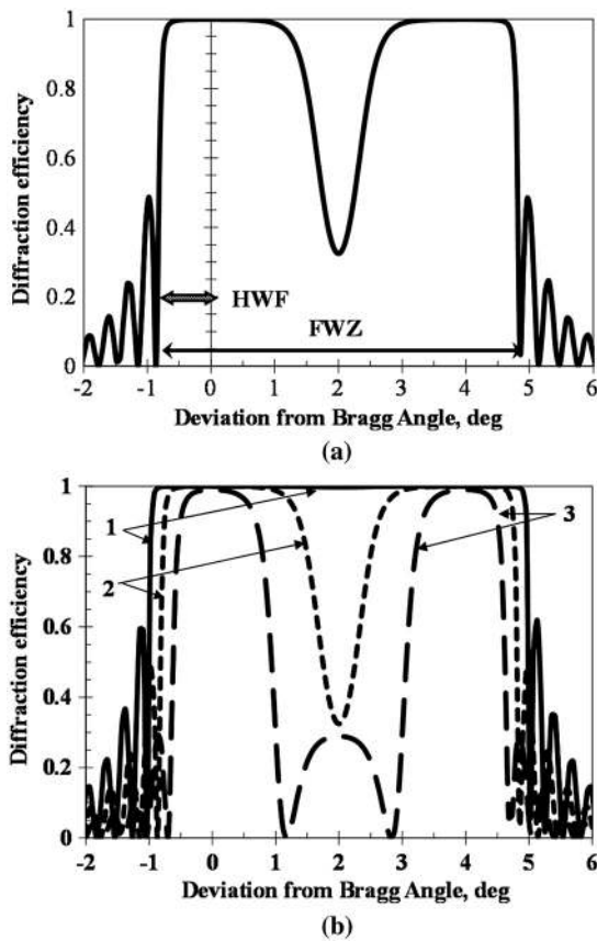
Fig. 5 Angular selectivity of 1-mm-thick reflecting VBG at \theta_m^* = 2^\circ . \lambda_0 = 1085 nm, n_{\text{av}} = 1.4867 . (a) Definition of angular selectivity at HWFZ (solid arrow) and FWZ (dashed arrow) levels. (b) Dependence of angular selectivity shape on refractive index modulation: 1 = 2000 ppm (solid line), 2 = 1500 ppm (dotted line), 3 = 1000 ppm (dashed line).
