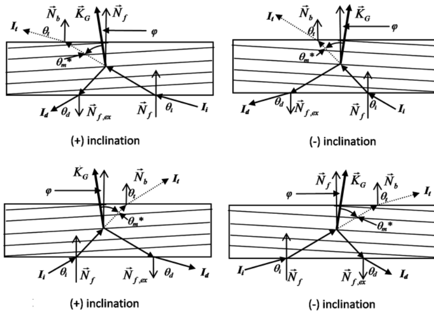
Fig. 2 Possible orders of Bragg diffraction for reflecting gratings with different angles of inclination. I_i, I_t, and I_d = incident, transmitted, and diffracted beams; \mathbf{K}_G = grating vector; \varphi = grating inclination; \theta_i, \theta_t, and \theta_d = angles of incidence, transmission, and diffraction; \theta_m^* = incident Bragg angle.
