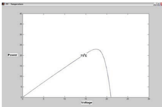
Fig. 12. Matlab model P-V curve for under conditions G= 1000 W/m^2 and T_p=75 ^{\circ}C .
