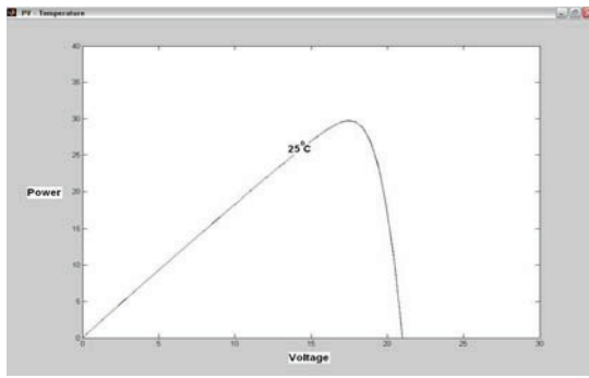
Fig. 10. Matlab model P-V curve for under conditions G=1000 W/m^2 and T_p=25 ^{\circ}C
