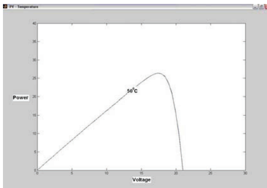
Fig. 11. Matlab model P-V curve for under conditions G=1000 W/m^2 and T_p=50 ^{\circ}C .
