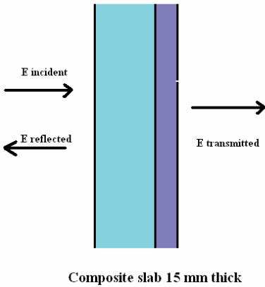
Figure 13. Stack of two composite layers: 12-mm absorbing layer (left) and 3-mm reflecting (right).
