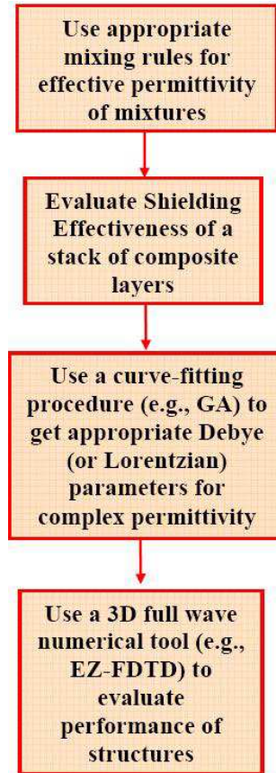
Figure 1. Design flowchart to design a shielding enclosure using composite materials.
